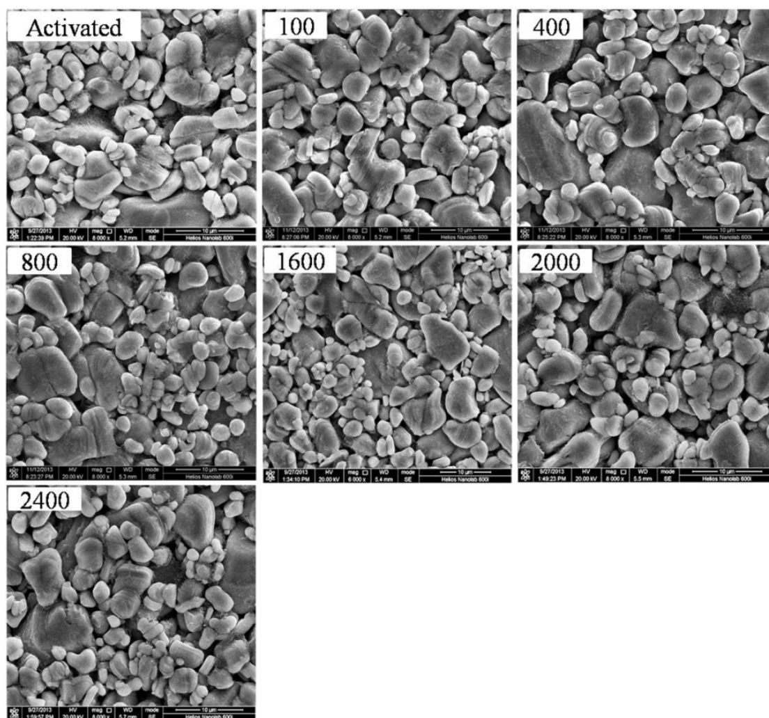
Fig. S1 SEM images of \text{LiCoO}_2 electrodes after different cycles (activated, 100 400, 800, 1600, 2000, 2400)
