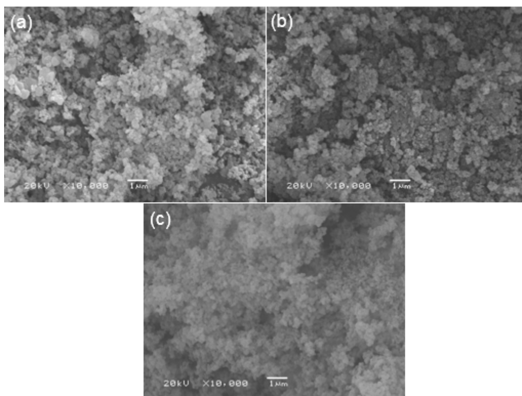
Fig. S1 the SEM images of the precursors tailoring with different Li:Mn:P molar ratio: (a) 2:1:1; (b) 2.5:1:1; (c) 3:1:1.
