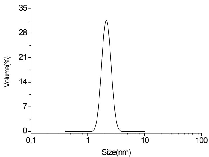
Fig. S2 DLS image of extractant phase of [Ch]Cl-methanol (20/80, mol/mol).
