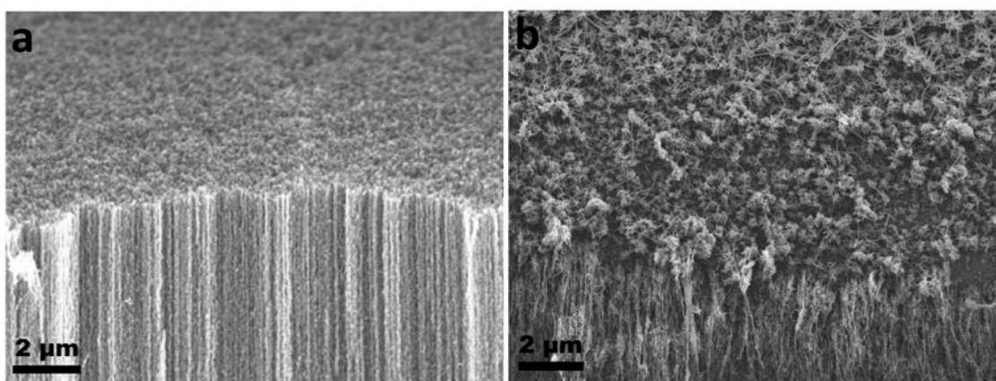
Fig. S1. SEM images of the working electrode before and after cycling measurements.
