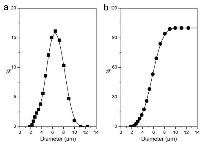
Fig. S1 The size distribution of the talc microparticles. Percentage of talc microparticles amount (a), Percentage of talc microparticles accumulated amount (b).
