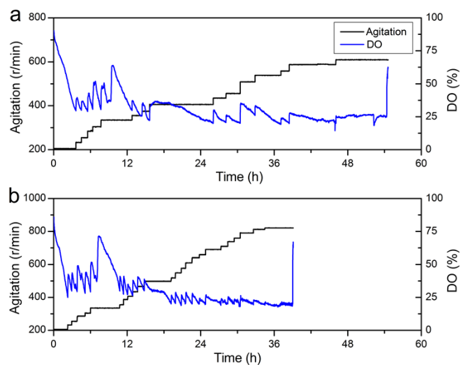
Fig. S2 Time courses of agitation speed and DO concentration in batch fermentations for \epsilon -PL production by Streptomyces sp. M-Z18 without (a) and with (b) talc microparticles (6 \mu m, 10 g/L).
