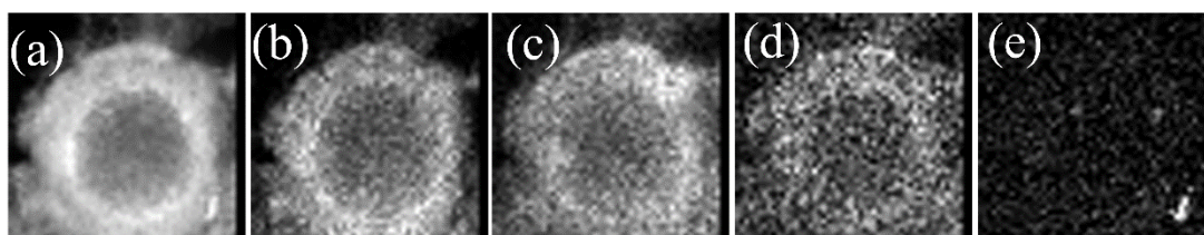
(a) the high angle annular dark field-scanning transmission electron microscopy (HAADF-STEM) image and mapping results of the elements (b) Ti, (c) O and (d) Fe (e) Ag for the Ag/ \gamma -Fe 2 O 3 @meso-TiO 2 .
