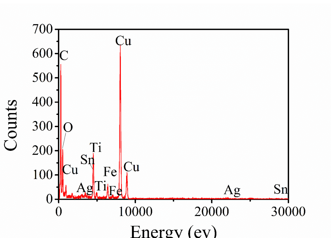
EDX of Ag/ \gamma -Fe 2 O 3 @meso-TiO 2
