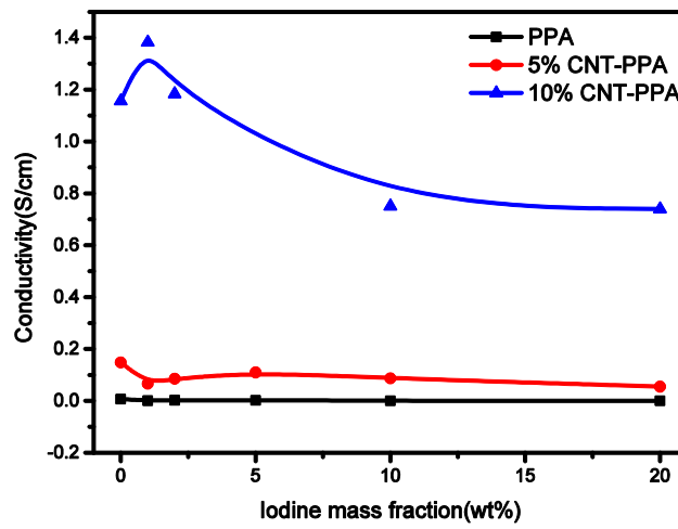
Figure S2. The conductivity of iodine-doped CNT-PPA composites
