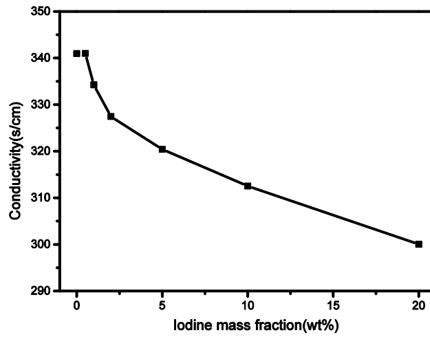
Figure S1. The conductivity of iodine-doped CNTs with the increasing mass fraction of iodine
