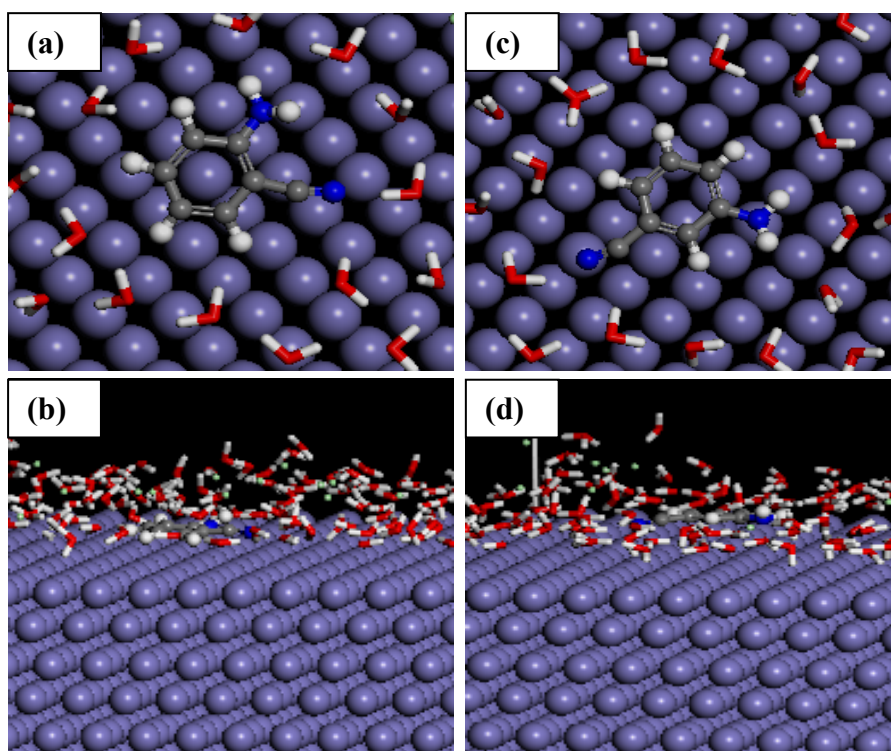
Fig. S3 Equilibrium adsorption configurations of inhibitors 2-AB (a and b) and 3-AB (c and d) on Fe (1 1 0) surface at 328 K obtained from MD simulations. Top: top view, Bottom: side view.
