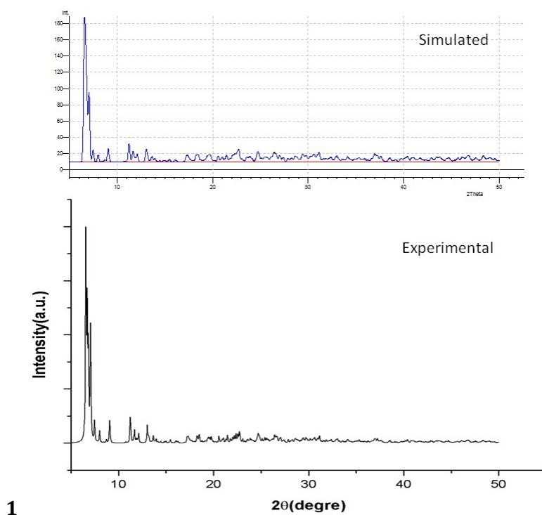
Figure S1. Experimental and simulated powder X-ray diffraction pattern of 1 .
