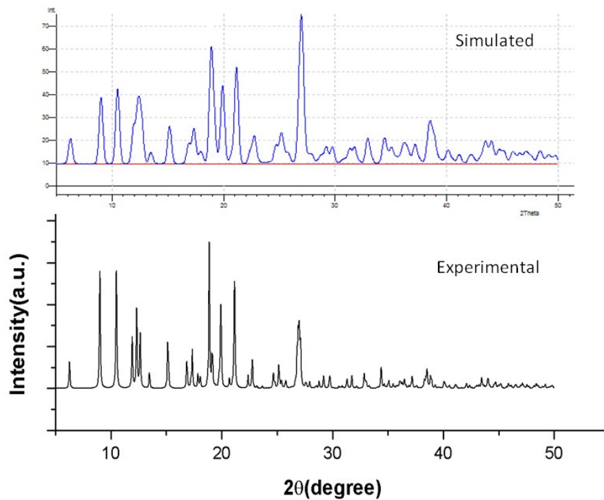
Figure S4. Experimental and simulated powder X-ray diffraction pattern of 4 .
