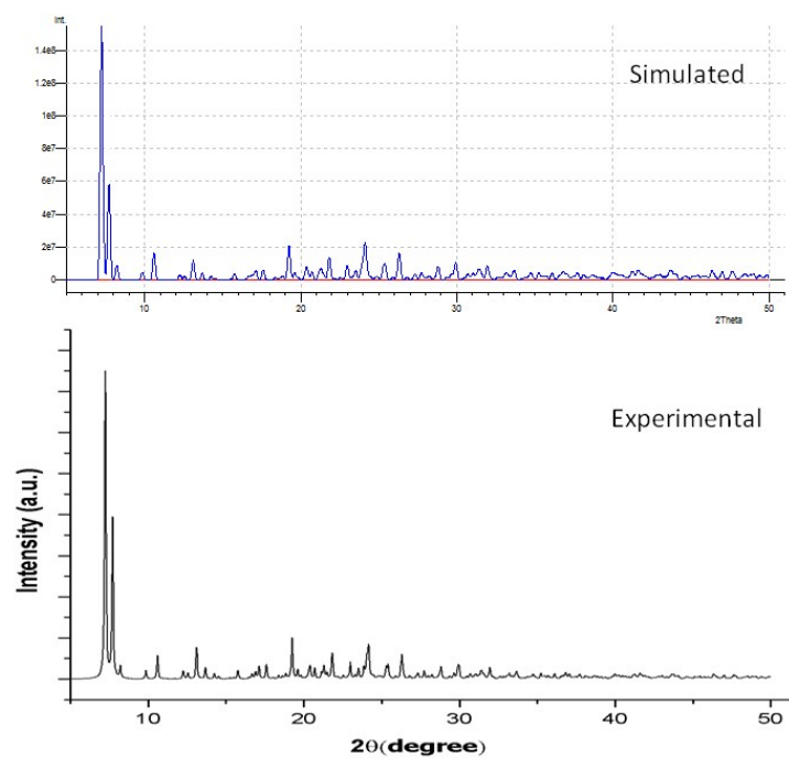
Figure S3. Experimental and simulated powder X-ray diffraction pattern of 3 .
