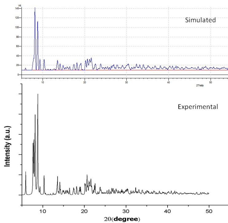
Figure S2. Experimental and simulated powder X-ray diffraction pattern of 2 .
