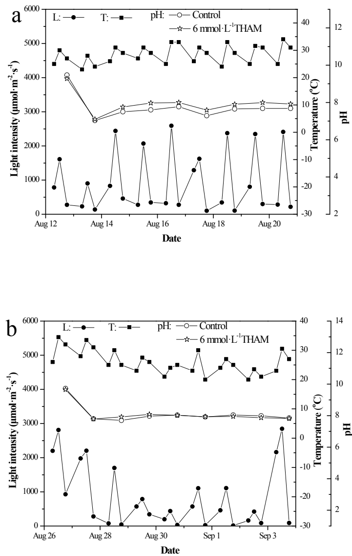
Fig. SM2 Light intensity, temperature, and pH versus time when S. dimorphus was cultured outdoors with different concentrations of THAM (0 and 6 mmol·L -1 ), 12 Aug. to 20 Aug. (a) and 26 Aug. to 3 Sep. (b)
