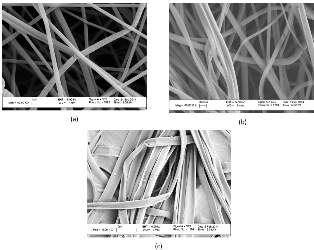
Fig. S1 SEM images of PMMA/PAAm/DCPD tri-axial healing fibers fabricated utilizing different outer wall solvents (a) and (b) DMF, and (c) ethyl acetate at lower magnifications.
