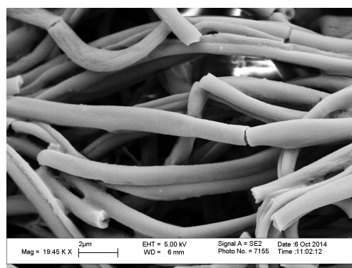
Fig. S2 SEM image of PMMA/PAAm/hardener tri-axial healing fiber at lower magnification
