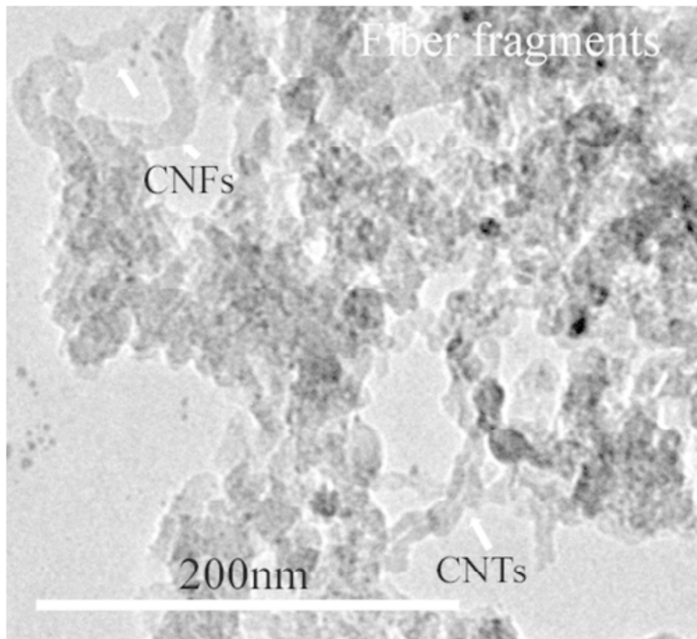
TEM images of final carbon products synthesized on carbon fibers at 550 °C with Ni used as catalyst 70x63mm (300 x 300 DPI)
