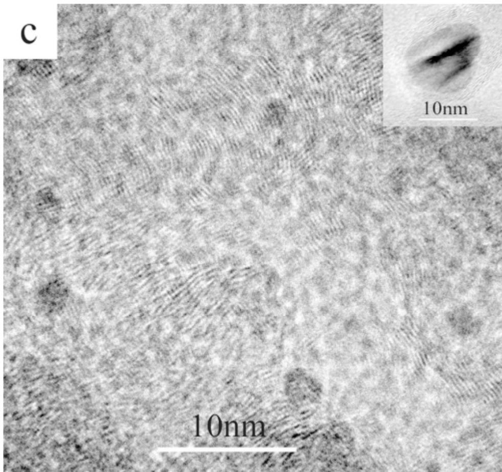
TEM images of catalyst particles after the CVD process performed at 600 °C with Ni used as catalyst 70x65mm (300 x 300 DPI)
