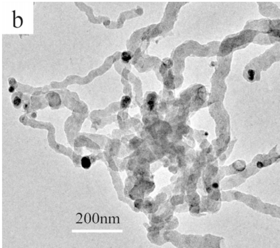
TEM images of catalyst particles after the CVD process performed at 500 °C with Fe used as catalyst 70x61mm (300 x 300 DPI)
