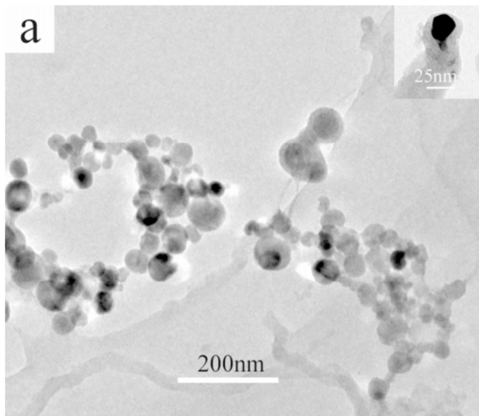
TEM images of catalyst particles after the CVD process performed at 500 °C with Ni used as catalyst 70x60mm (300 x 300 DPI)
