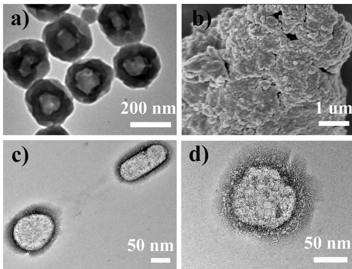
Figure S1 The SEM and/or TEM photos of a) polymer spheres and b, c and d) carbon spheres
