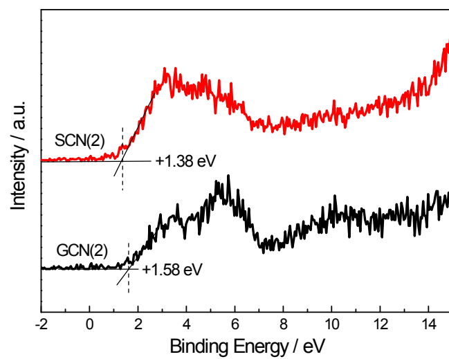
Figure S4. VB XPS of as-prepared GCN(2) and SCN(2).
