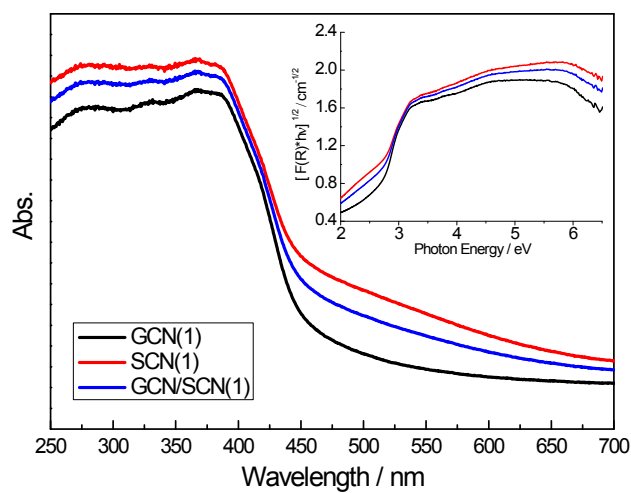
Figure S1. UV-Vis spectra of the as-prepared GCN(1), SCN(1) and GCN/SCN(1).
