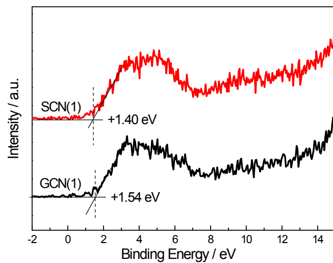
Figure S3. VB XPS of as-prepared GCN(1) and SCN(1).
