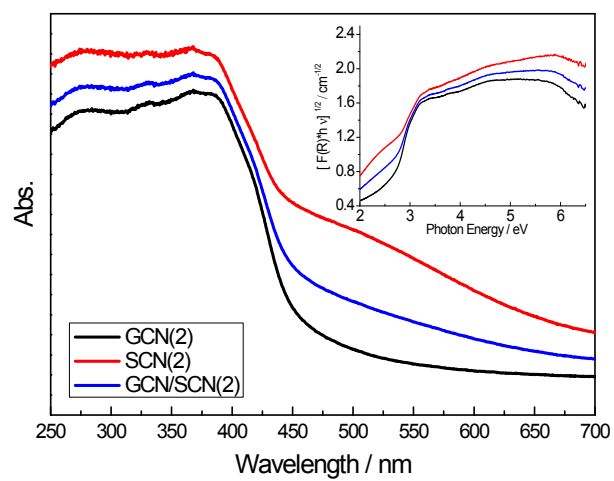
Figure S2. UV-Vis spectra of the as-prepared GCN(2), SCN(2) and GCN/SCN(2).
