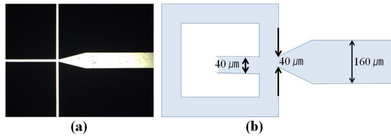
Figure SI 1. (a) Camera image and (b) schematic diagram showing the dimensions of the microfluidics channels.
