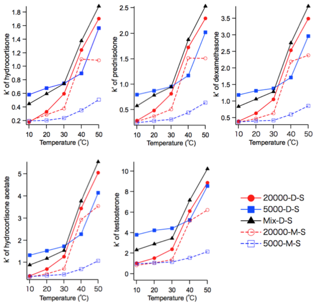
Fig. S2 Temperature dependent retention factors of steroids on HPLC column: (a) hydrocortisone, (b) prednisolone, (c) dexamethasone, (d) hydrocortisone acetate, and (e) testosterone.
