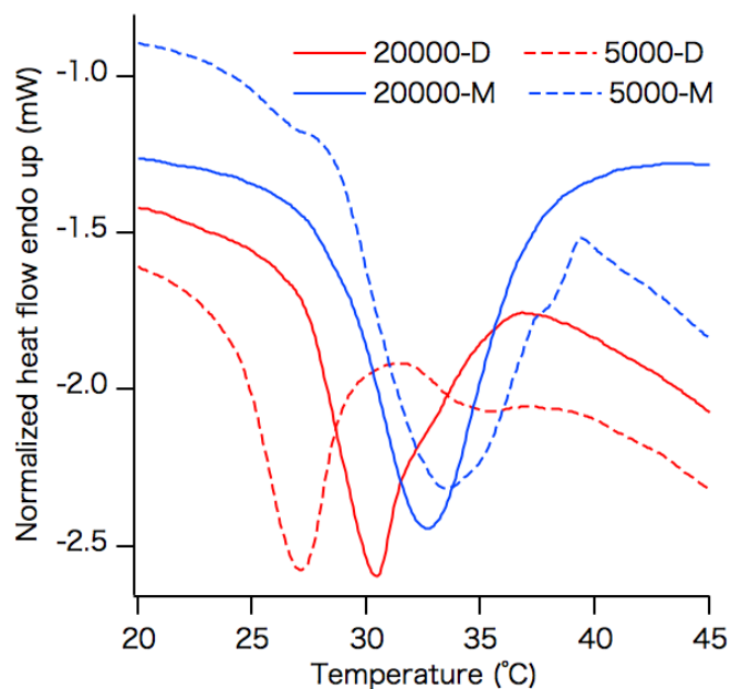
Fig. S1 Microcalorimetric endotherm of polymers in water.
