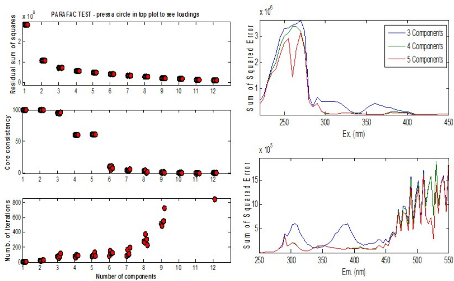
Fig. 1 Results of core consistency and sum of squared error
