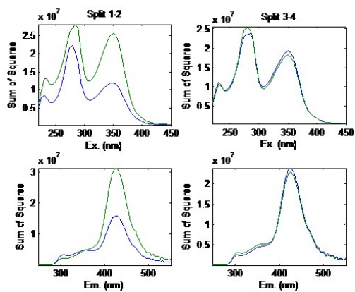
Fig. 2 Results of split half analysis
