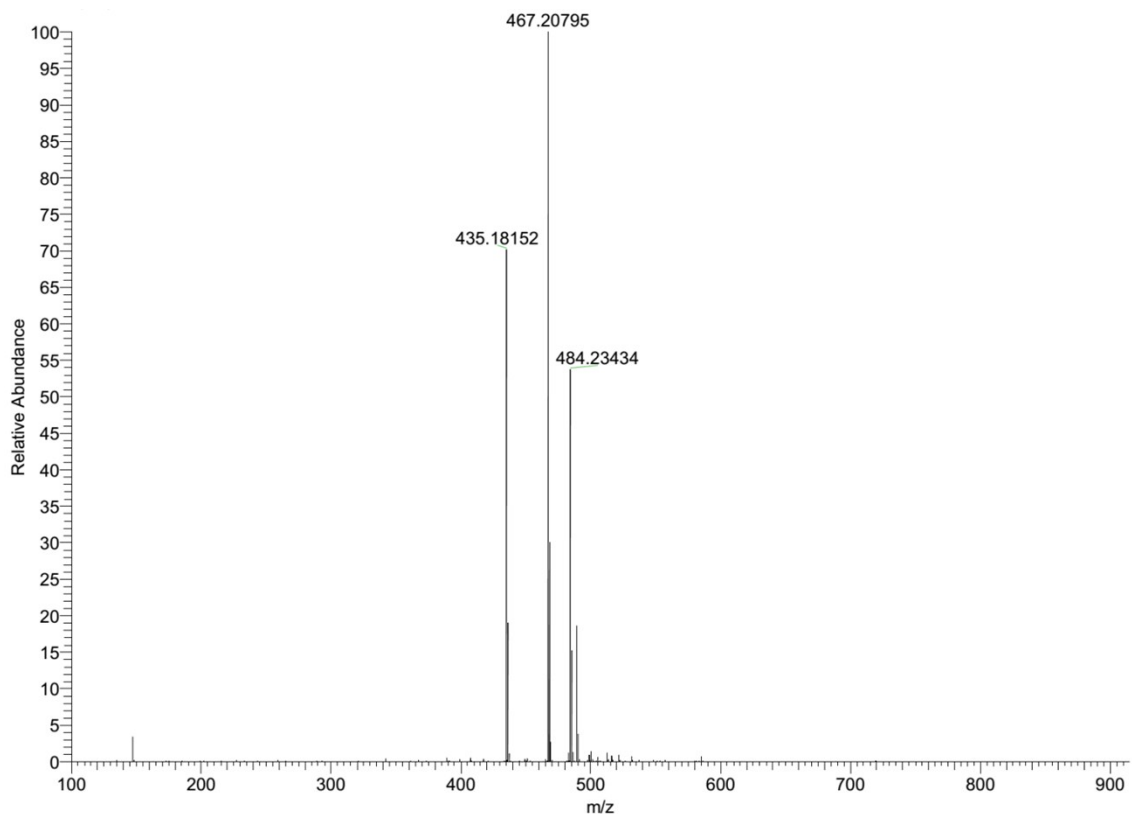
Mass spectrum of nimbolide
