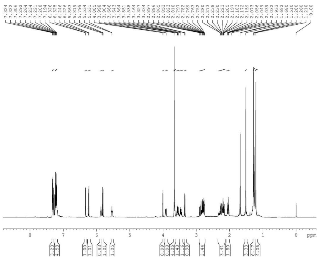
1 H NMR Spectrum of 1c
