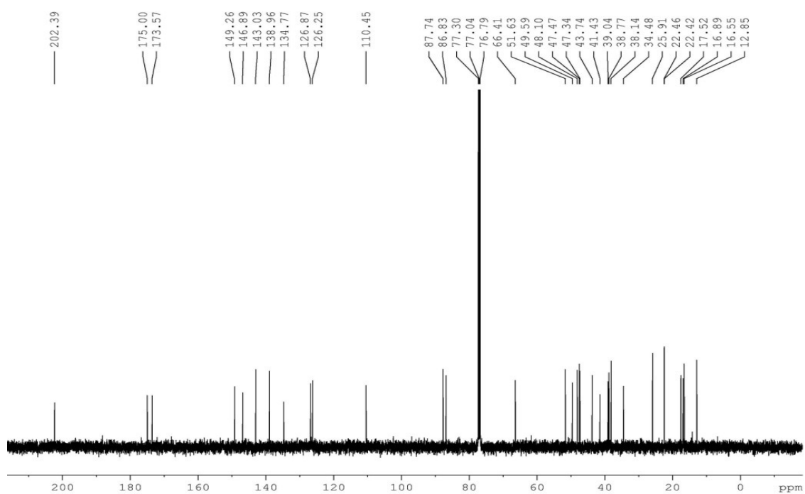
13 C NMR Spectrum of 1b
