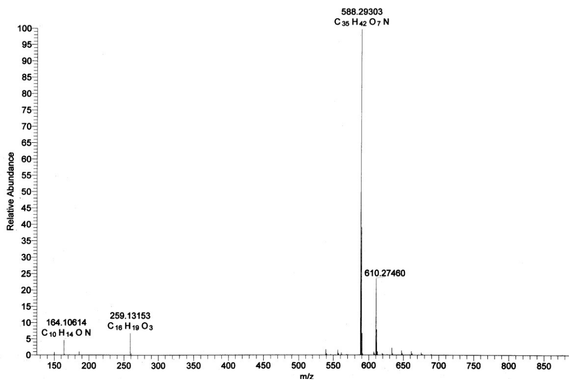
Mass Spectrum of 1c
