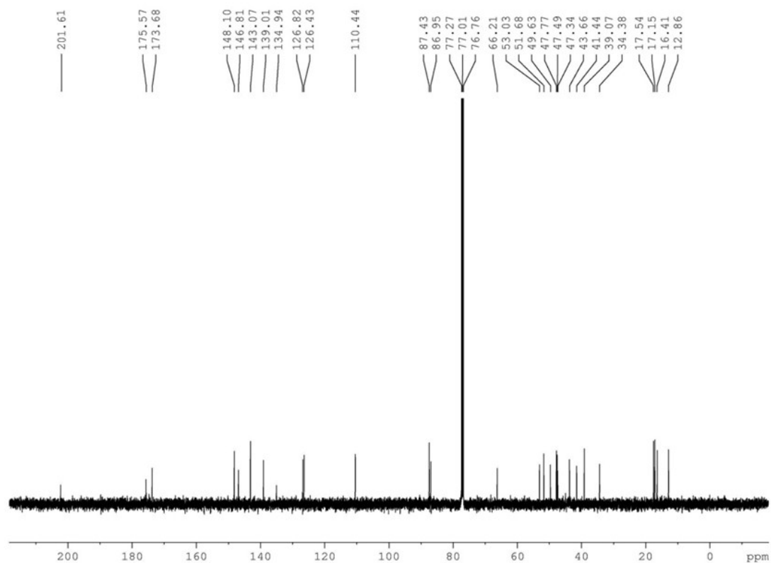
13 C NMR spectrum of desacetylnimbin
