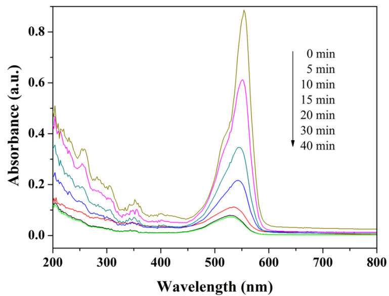
Fig. S1. Temporal UV–vis absorption spectral changes of RhB solution during the photodegradation process over 3% BiPO 4 /Bi 2 O 2 CO 3 .
