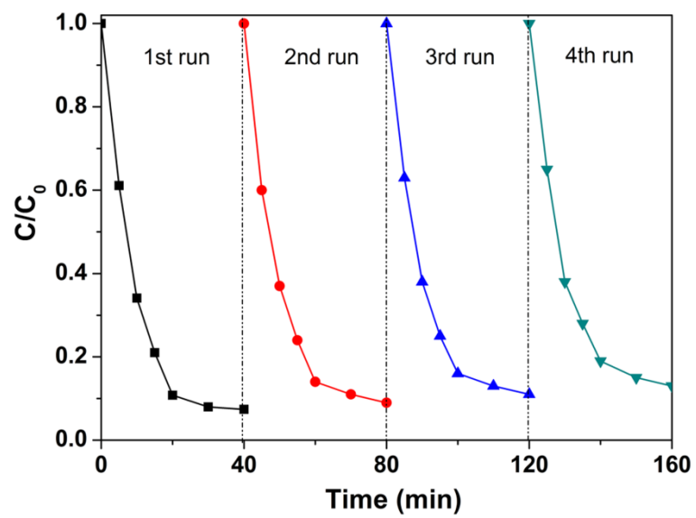
Fig. S2. Cycling runs of RhB degradation over 3% \text{BiPO}_4/\text{Bi}_2\text{O}_2\text{CO}_3 .
