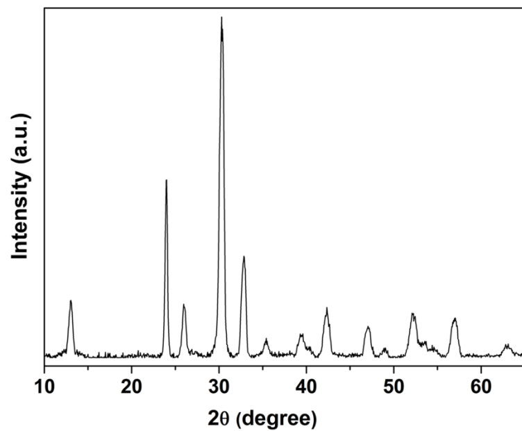
Fig. S3. XRD pattern of 3% BiPO 4 /Bi 2 O 2 CO 3 after four cycling runs.
