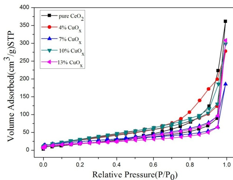
Figure.S3.N 2 adsorption-desorption isotherms of CuO x -CeO 2 composite hollow sphere
