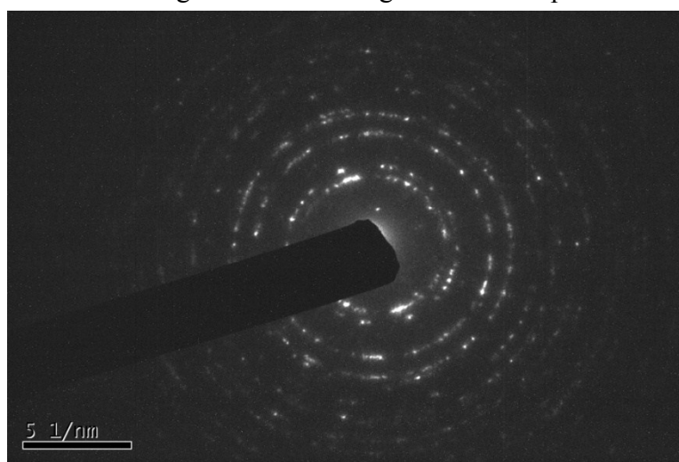
Figure.S2.SEAD patterns of 10%CuO x -CeO 2 composite hollow spheres
