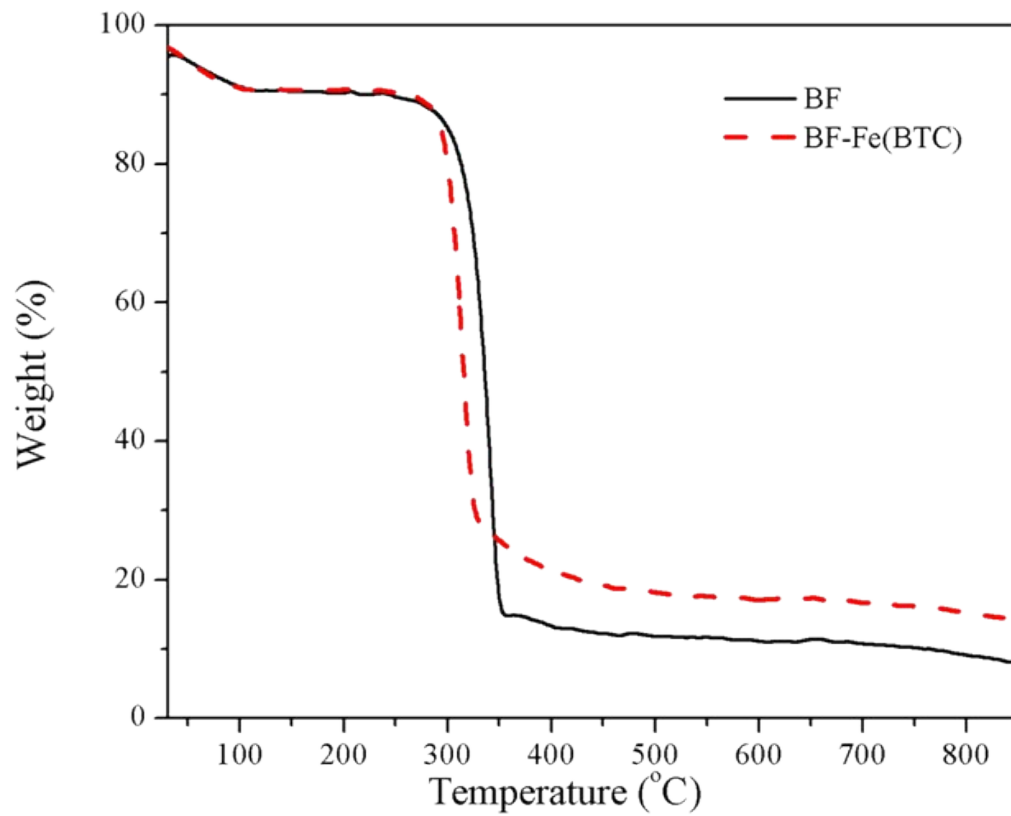
Fig. S1 TGA thermograms of BF and BF-Fe(BTC).
