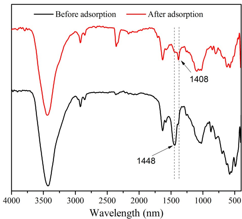
Fig. S2 FT-IR spectra of MBF-900 and MBF-900.
