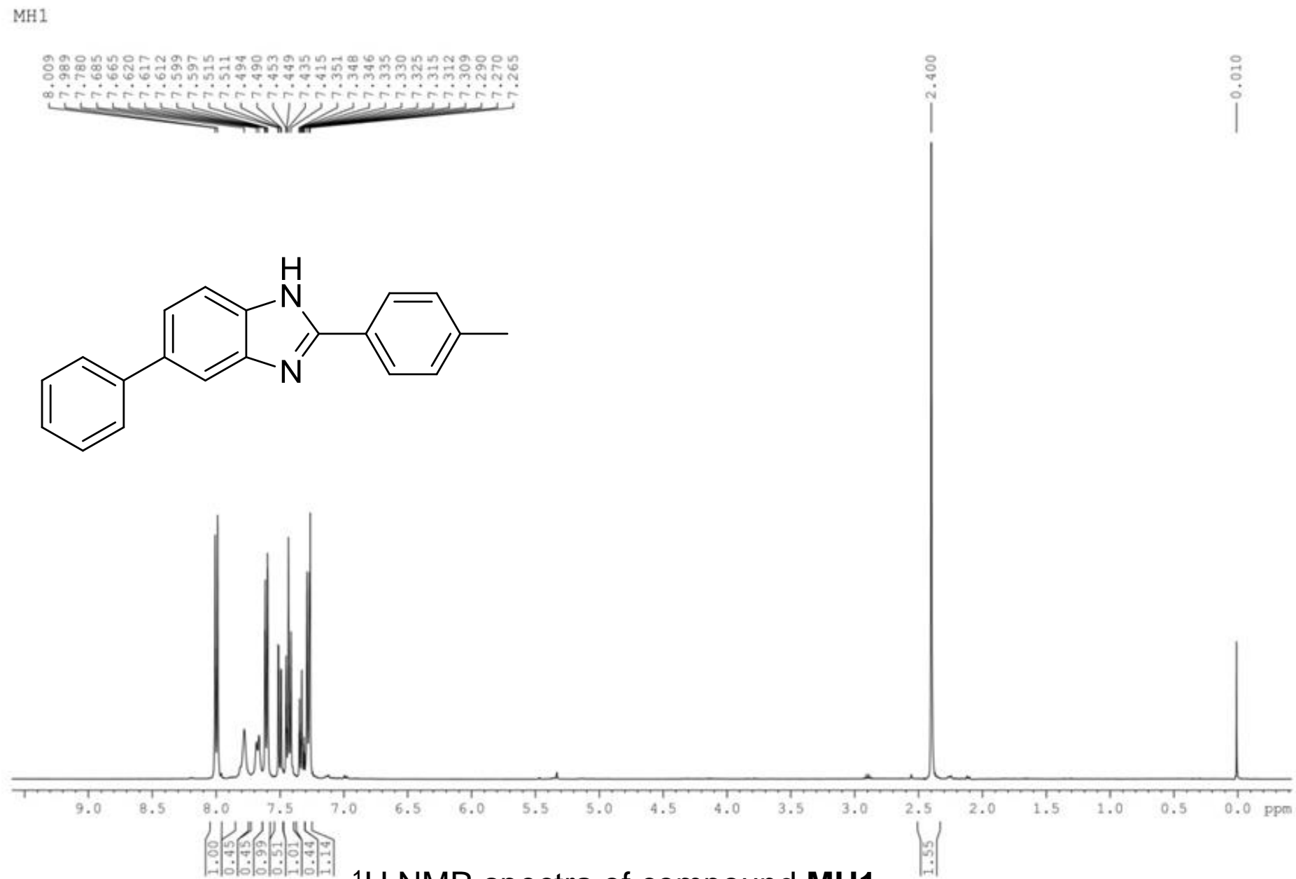
^1\text{H} NMR spectra of compound MH1
