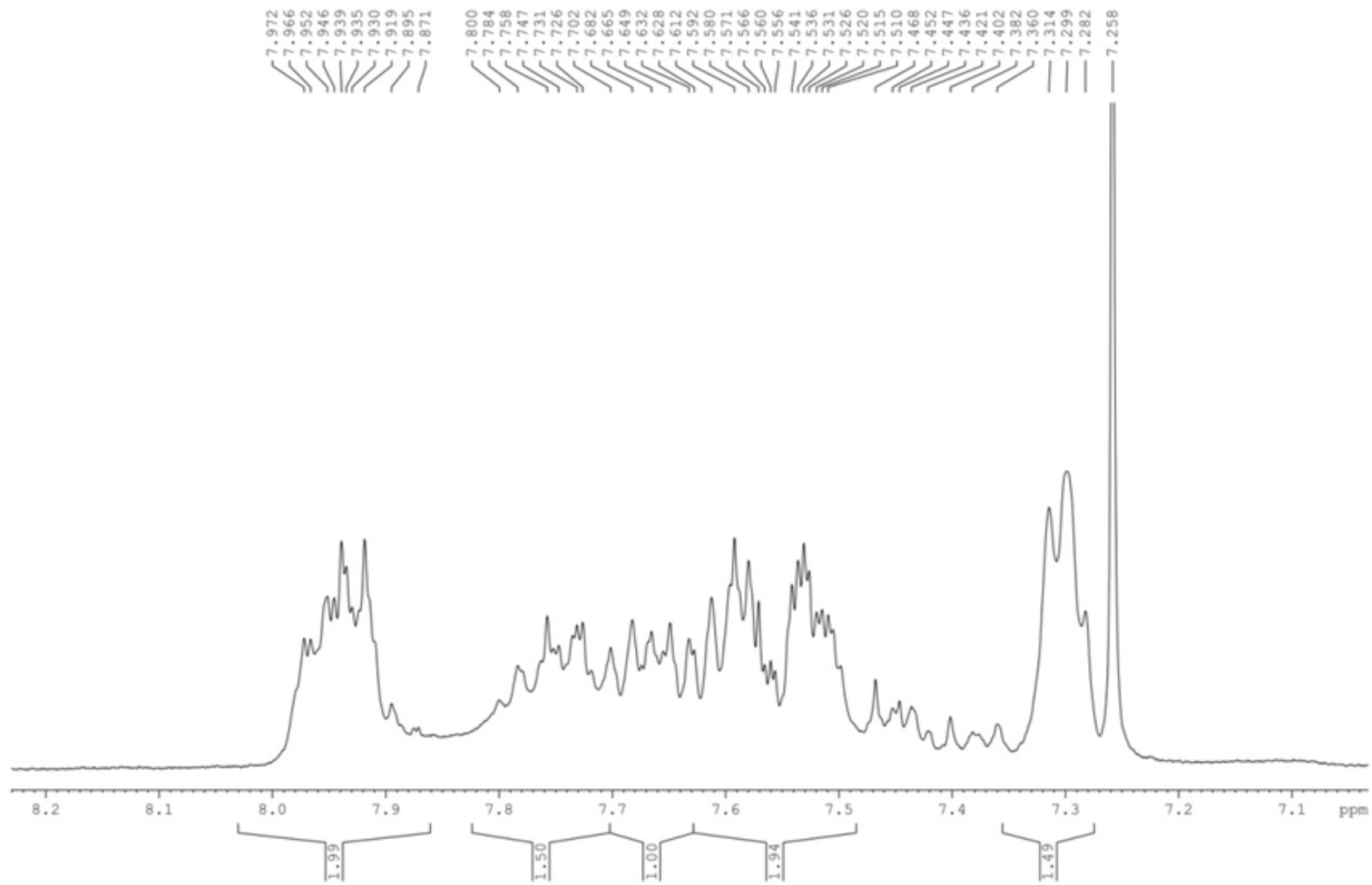
^1\text{H} NMR spectra of compound MH5 extended
