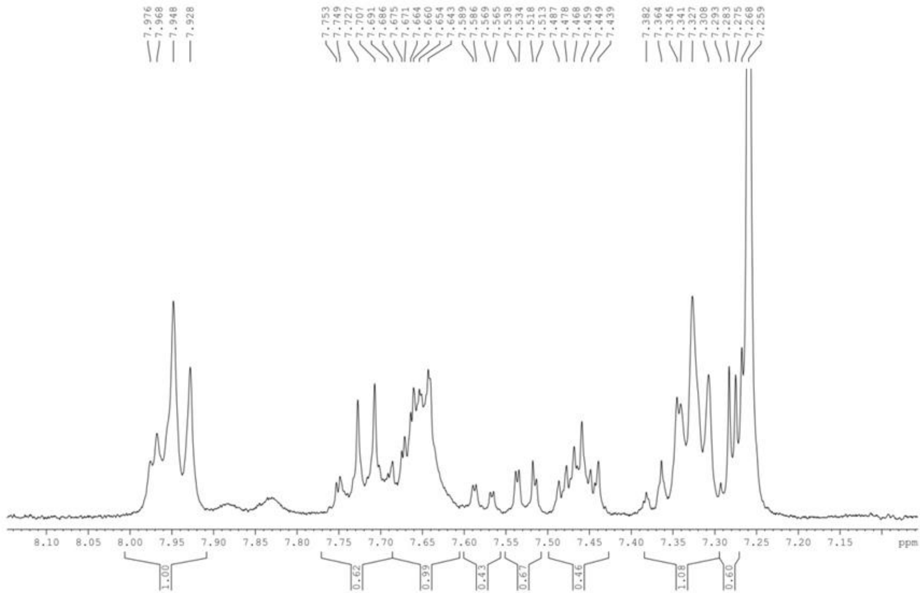
^1\text{H} NMR spectra of compound MH2 extended
