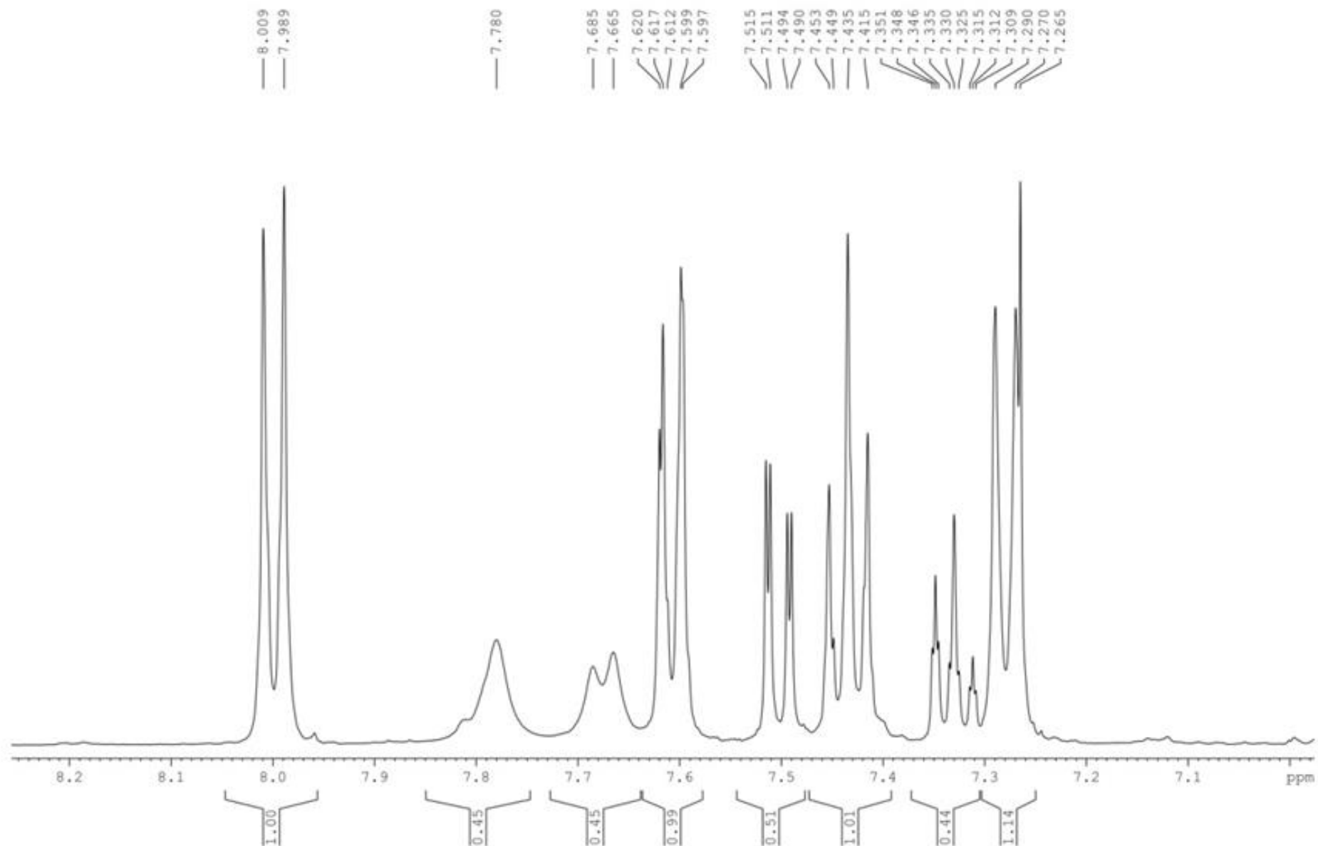
1 H NMR spectra of compound MH1 extended
