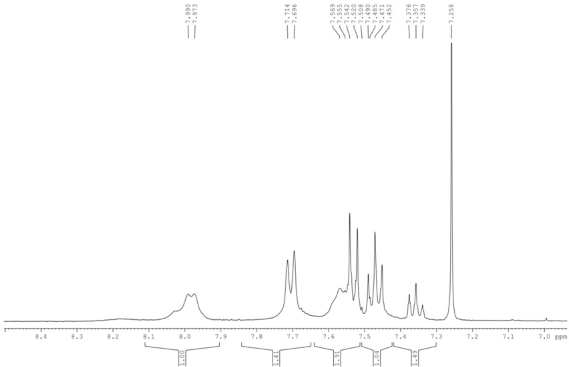
^1\text{H} NMR spectra of compound MH4 extended
