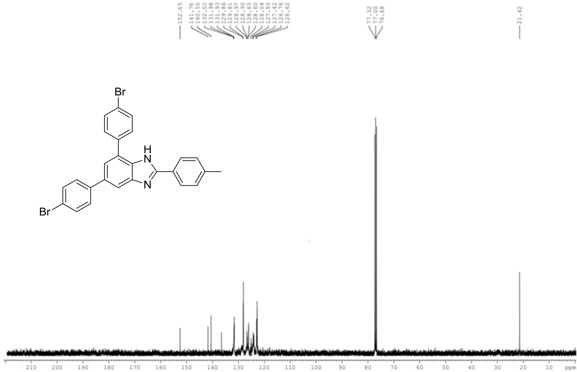
13 C NMR Spectrum of compound MH4
