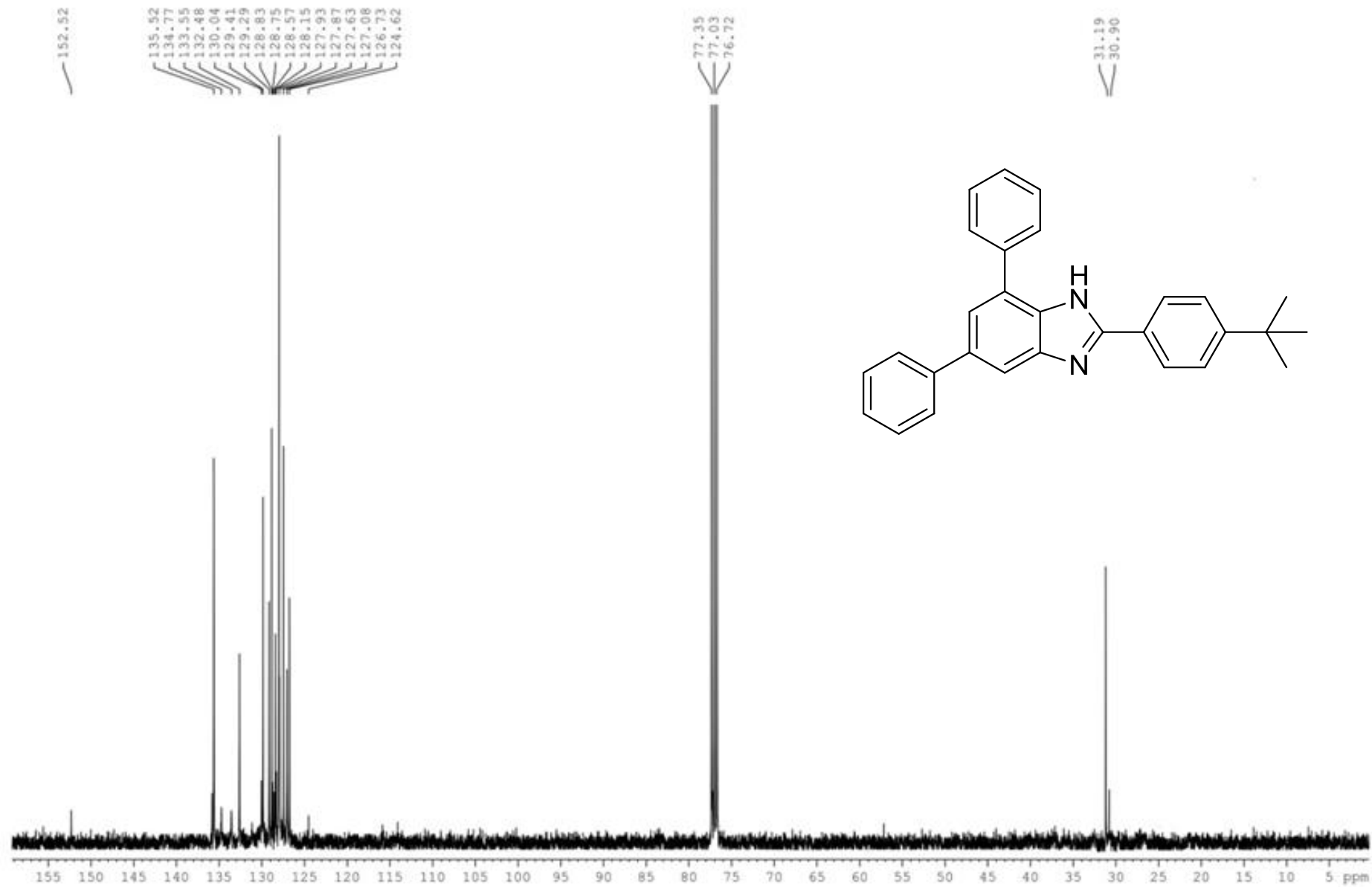
^{13}\text{C} NMR Spectrum of compound MH5
