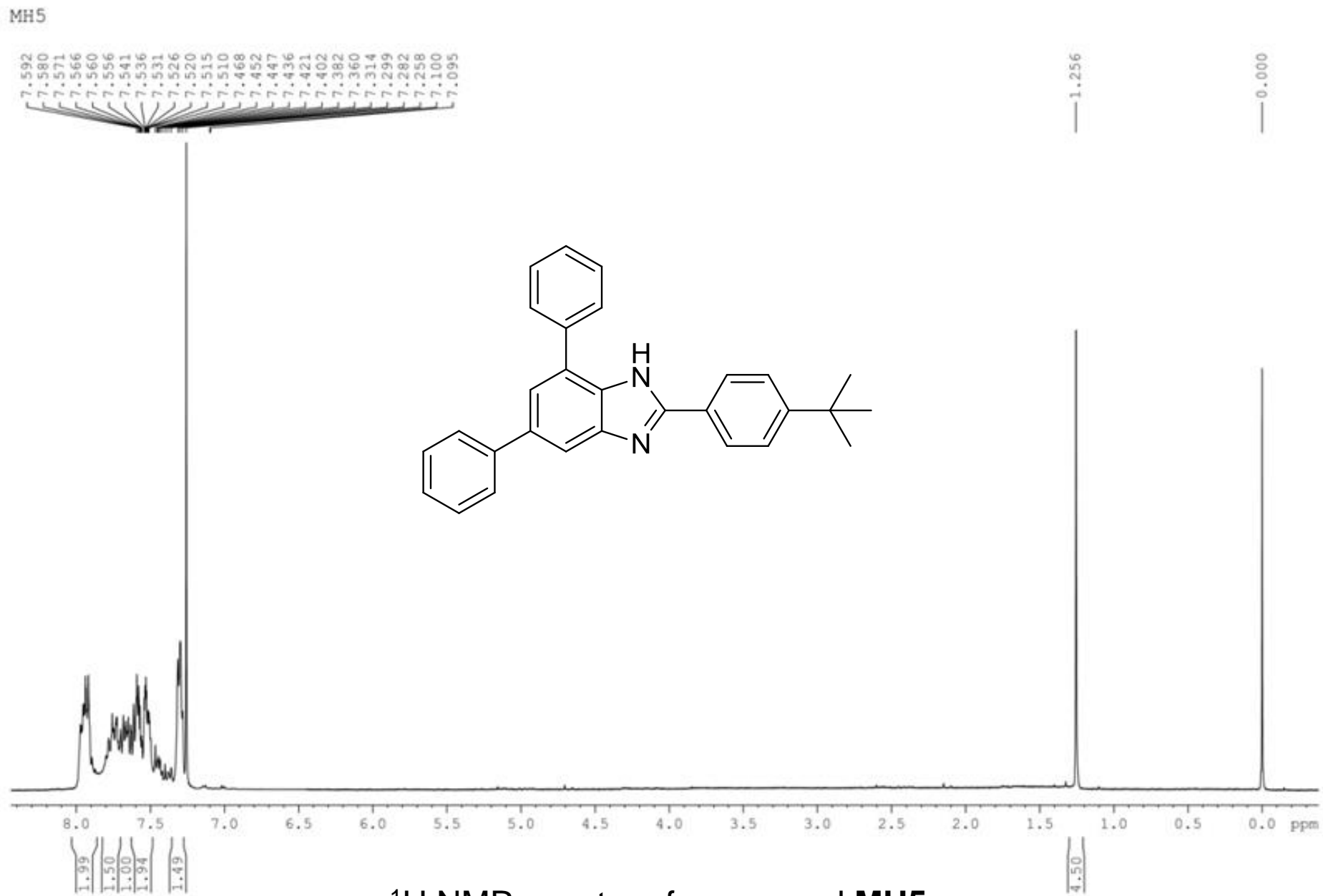
^1\text{H} NMR spectra of compound MH5
