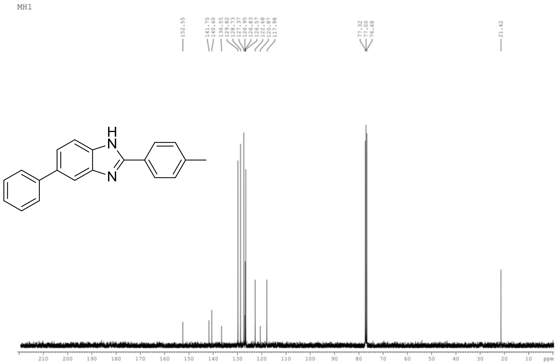
^{13}\text{C} NMR Spectrum of compound MH1
