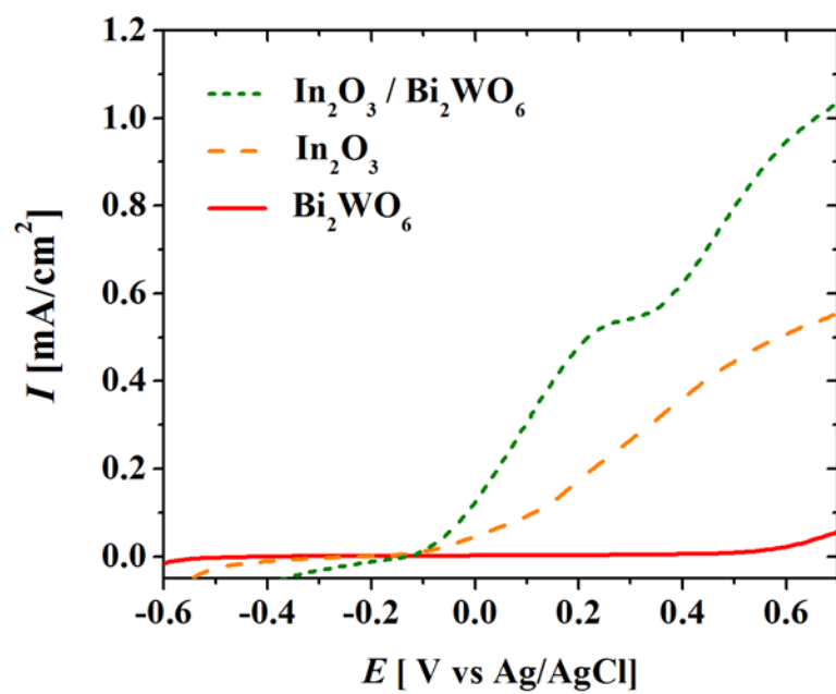
Figure S2 photocurrent of individual layers of Bi80, In24 and Bilayer In24-Bi80 film
