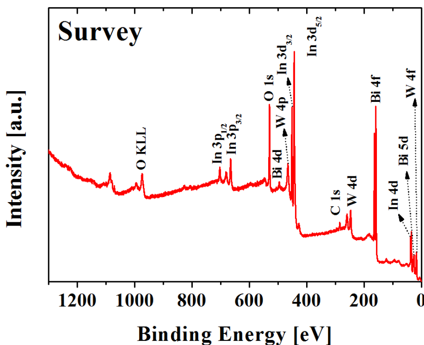
Figure S1 XPS survey spectra of Bilayer In 24 -Bi 80 film
