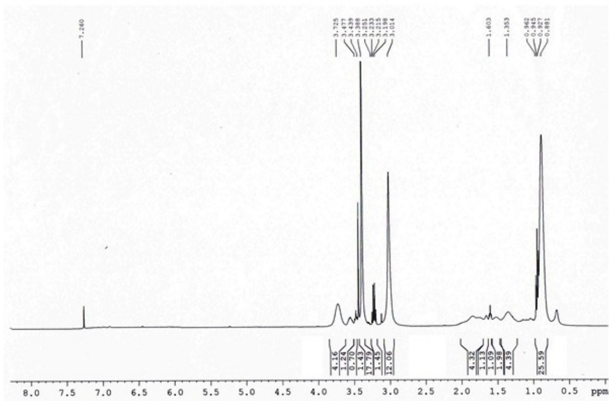
Figure S1: 1 H NMR of CLPN-1 in CDCl 3 .
