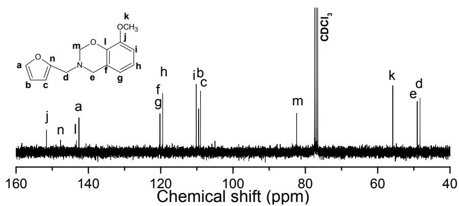
Figure S4 ^1\text{H} -NMR and ^{13}\text{C} -NMR spectra of Bz_Gf .
