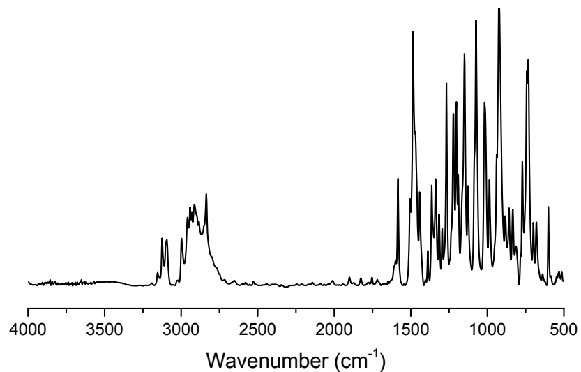
Figure S3 FT-IR spectrum of Bz_Gf .
