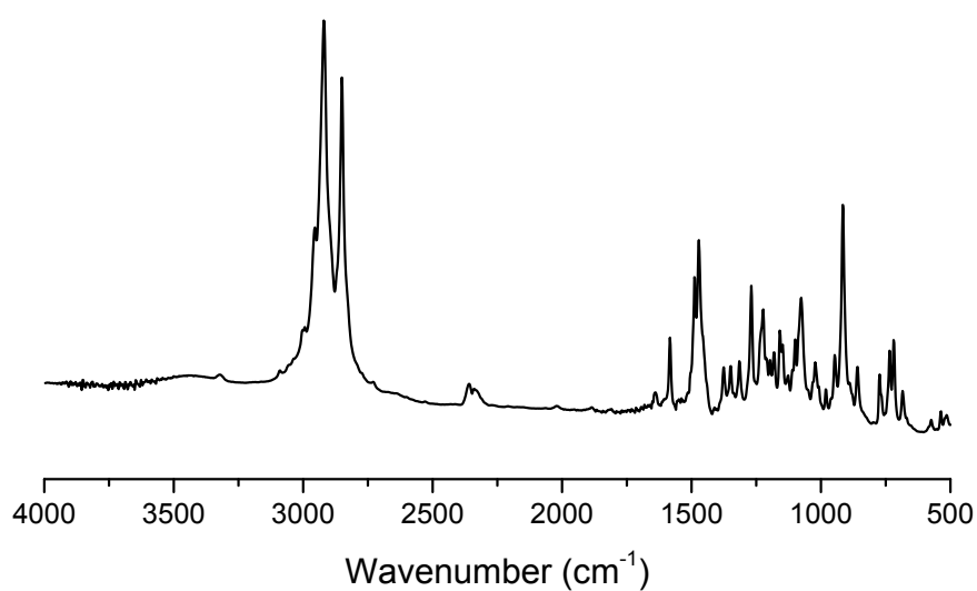
Figure S1 FT-IR spectrum of Bz_Go .
