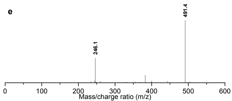
Figure S5 MALDI mass of (a1) TP (positive mode), (a2) TP (negative mode), (b) Bz_TPo (positive mode), (c) Bz_TPf (positive mode), (d) Bz_Go (positive mode) and (e) Bz_Gf (positive mode).
