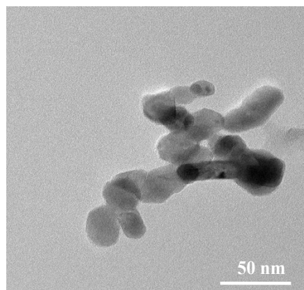
Fig.S1. TEM image of LaFeO 3 NPs synthesized by ILS (50 mM) assisted hydrothermal route.
