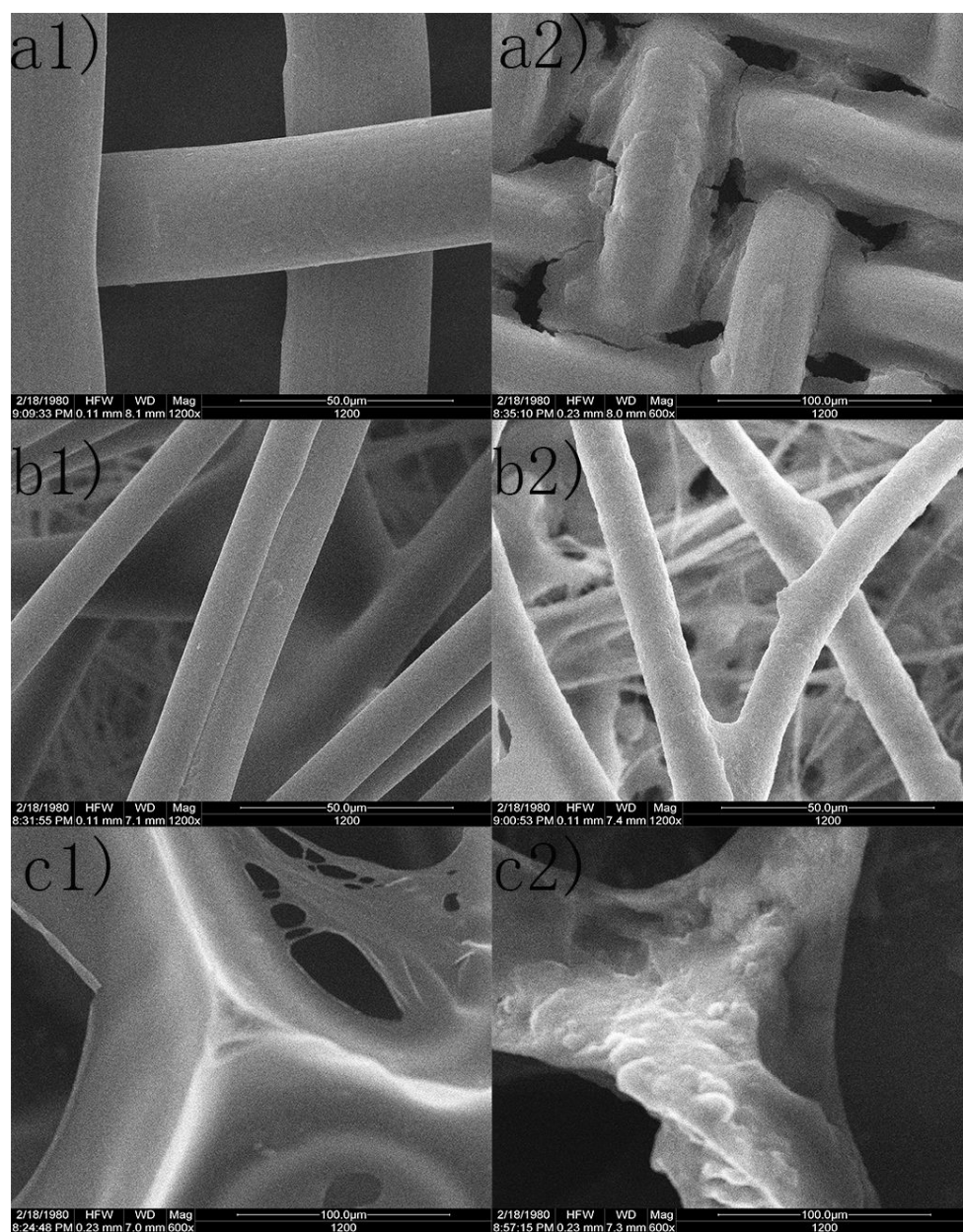
S4: Figures of original materials (copper mesh a1, filter paper b1, sponge c1), and coatings after water jetting tests (copper mesh a2, filter paper b2, sponge c2).
