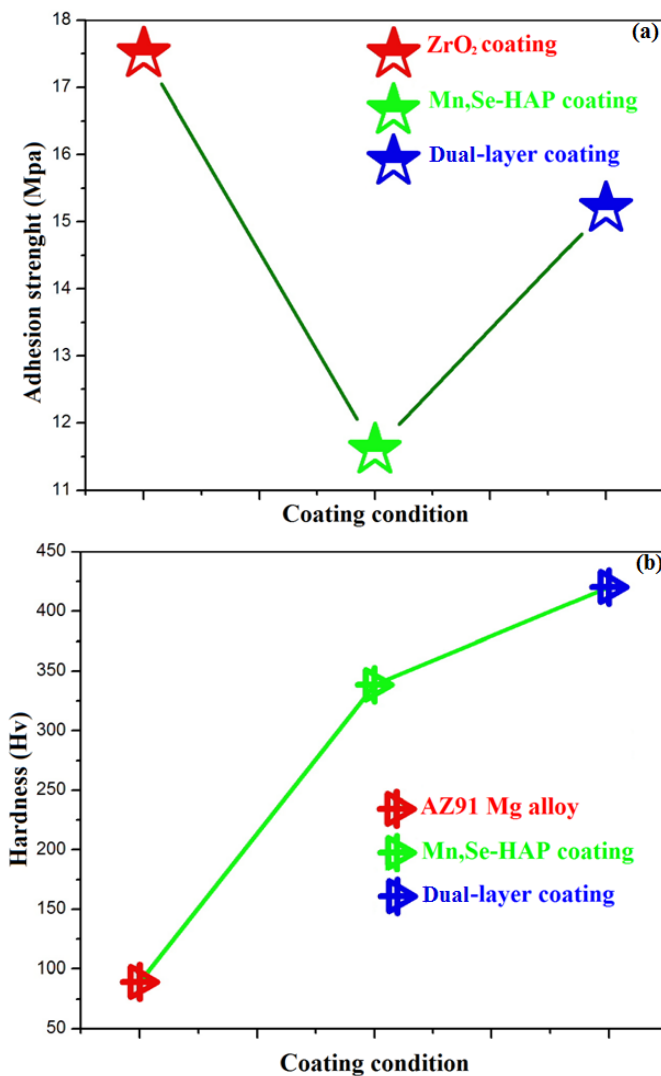
Fig. S1 (a) Adhesion strength of ZrO 2 , Mn,Se-HAP, and dual layer coating and (b) Hardness of AZ91 Mg alloy, Mn,Se-HAP and dual layer coating.
