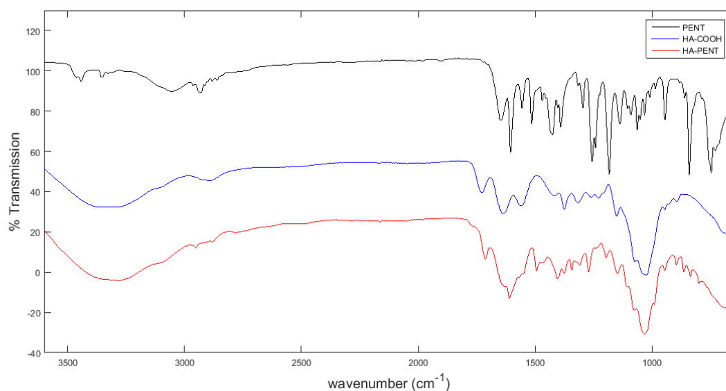
Figure S1 . FT- IR Spectra of Pent, HA-COOH and HA-Pent
