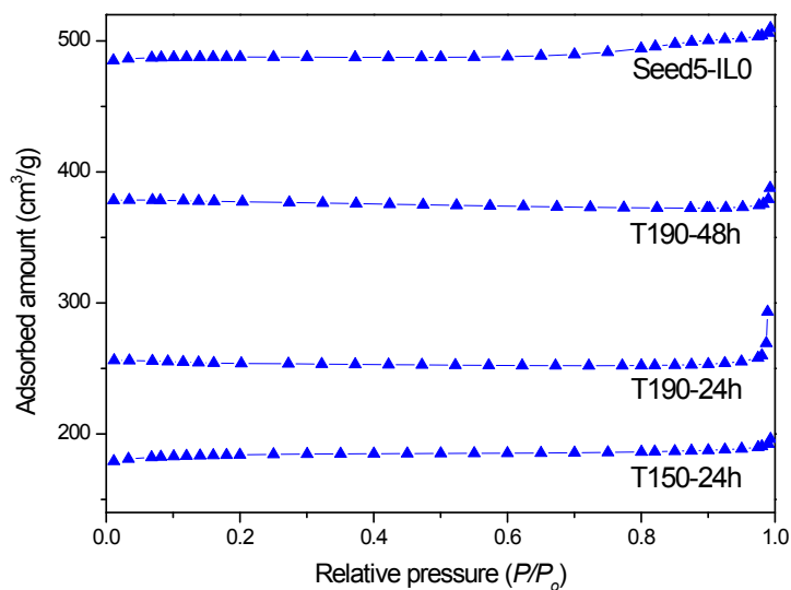
Fig. S1 N 2 adsorption isotherms of the calcined samples T150-24h, T190-24h, T190-48h and Seed5-IL0 (The isotherms for T190-24h, T190-48h and Seed5-IL0 were offset vertically by 100, 200 and 300 cm 3 /g).
