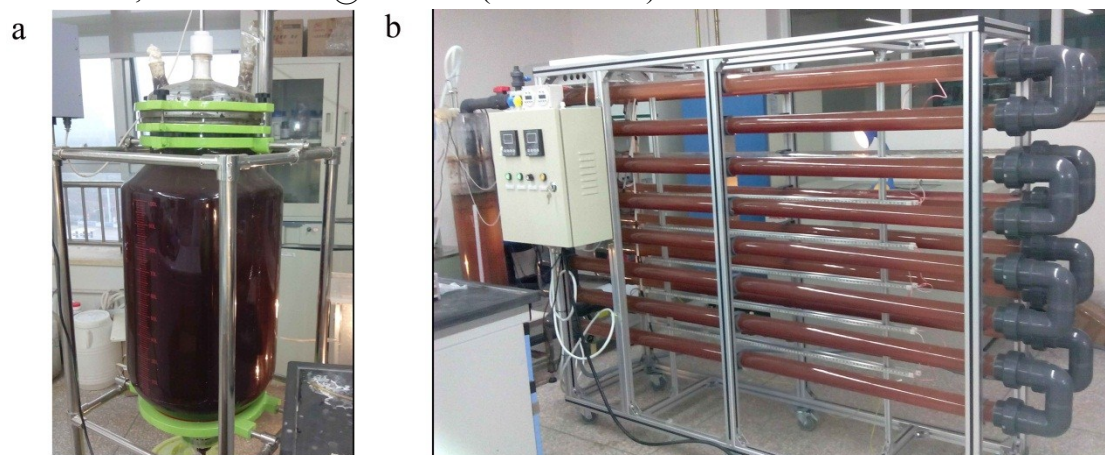
Fig. S1. Photograph of the CSTR (a) and TPBR (b).
