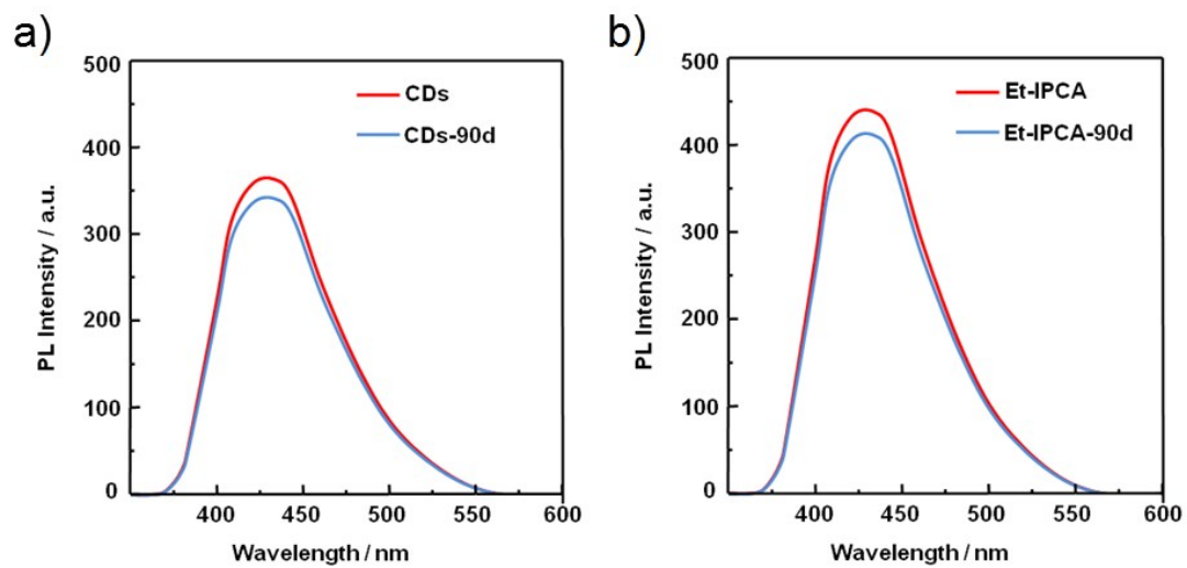
Fig. S1 PL images and photostability data for the CDs and Et-IPCA stored at room temperature.
