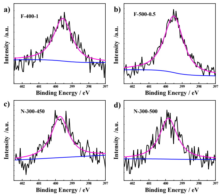
Figure S1. N1s XPS spectra of the carbon doped photocatalysts.
