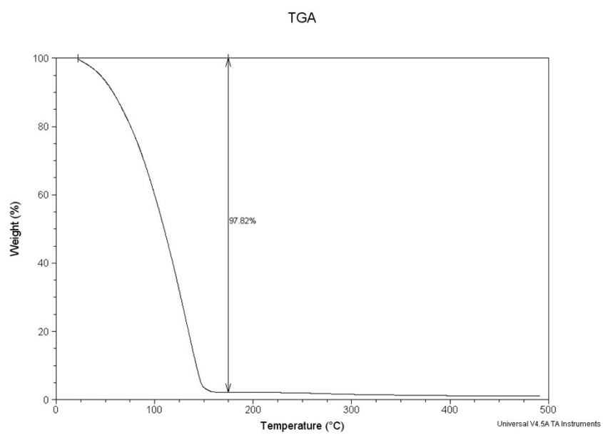
Fig.S5 TGA curve of calcium PPOR-alginate hydrogel
