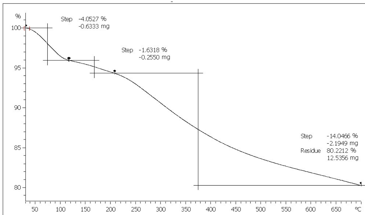
Fig. S1. TGA of 1 .
