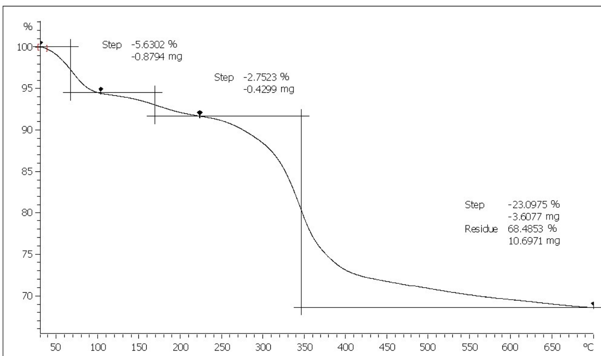
Fig. S2. TGA of 3 .
