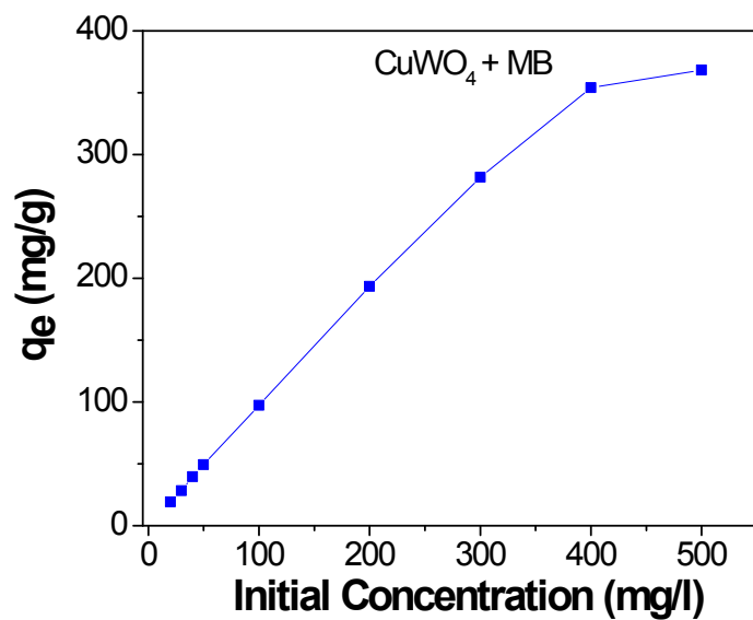
Figure S2: The extent of sorption of MB dye (pH = 3) by 10mg \text{CuWO}_4 nanoparticles as a function of the initial dye concentration.
