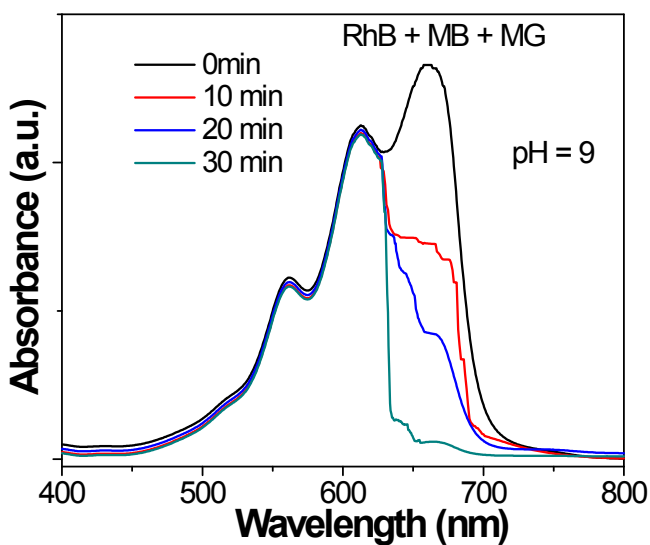
Figure S1: Selective sorption of MB dye from 20ppm mixture of RhB, MB and MG by \text{CuWO}_4 nanoparticles at pH = 9.
