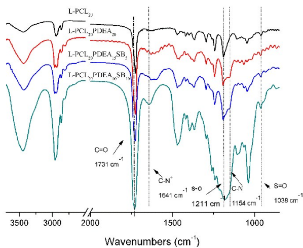
Figure S1. FT-IR spectra for PCL, PCL-PDEA and PCL-PDEASB.
