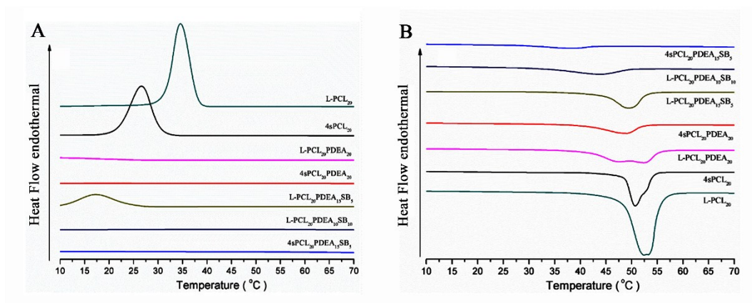
Figure S2. The DSC curves of PCL, PCL-PDEA and PCL-PDEASB.
