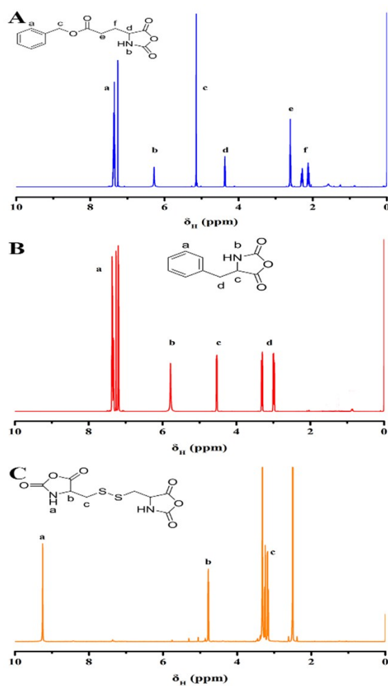
Fig. 2S ^1\text{H} NMR spectrum of BLG-NCA (A, \text{CDCl}_3 ), Phe-NCA (B, \text{CDCl}_3 ) and Cys-NCA (C, \text{DMSO-d}_6 ).
