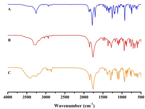
Fig. 1S FT-IR spectra of BLG-NCA (A), Phe-NCA (B) and Cys-NCA (C).
