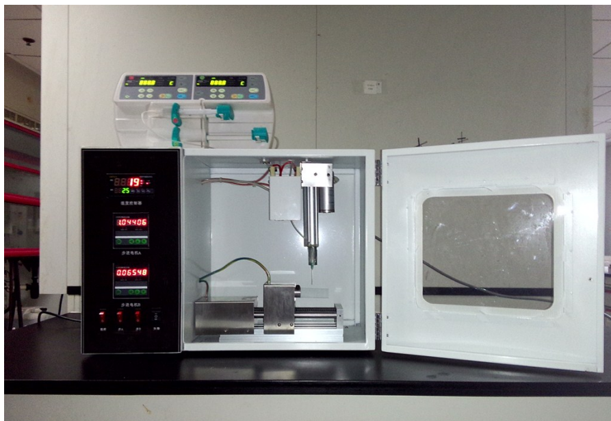
Fig. S1 Panoramic image of experimental platform including microfluidic spinning machine, microfluidic pump, syringes, microchannel, 20G stainless steel needle.
