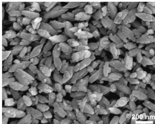
Fig. S1 SEM image of spindle-like \text{LiMnPO}_4 prepared with CA-free precursor.
