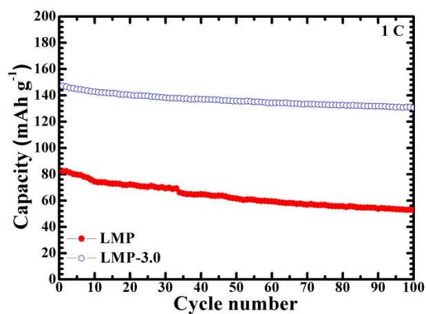
Fig. S2 Comparison of cycling stability of spindle-like \text{LiMnPO}_4 and LMP-3.0.
