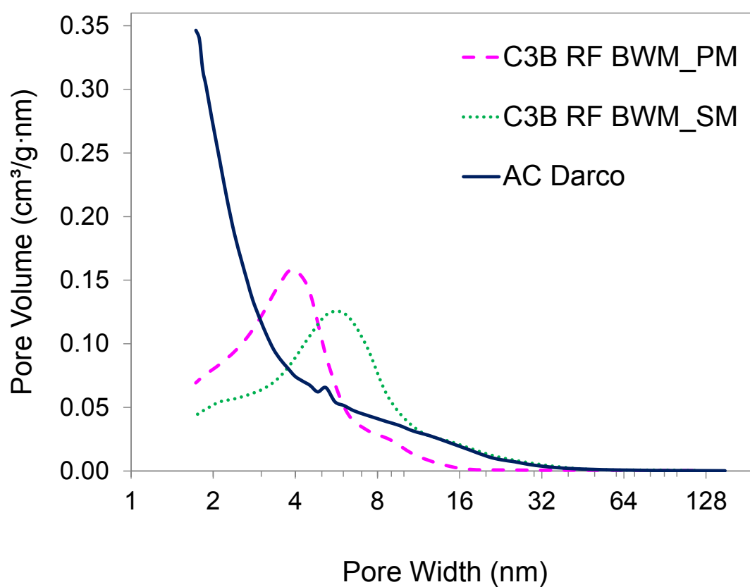
Figure S.1. Pore size distribution of nanocarbons (C3BRFBWM_PM and C3BRFBWM_SM) and commercial activated carbon (AC Darco)
