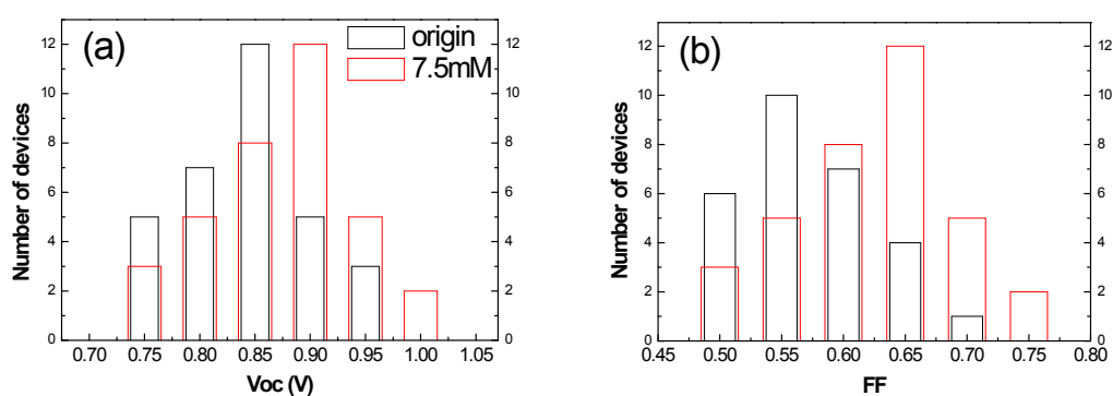
Figure S1. The V_{oc} (a) and FF (b) distribution of the perovskite photovoltaic cells with or without amino-silane modification.
