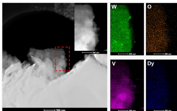
Fig. S2 The TEM-mapping images of DyVO 4 /WO 3 films
