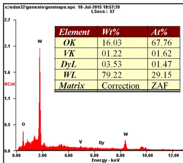
Fig. S1 The EDS spectra of DyVO 4 /WO 3 films
