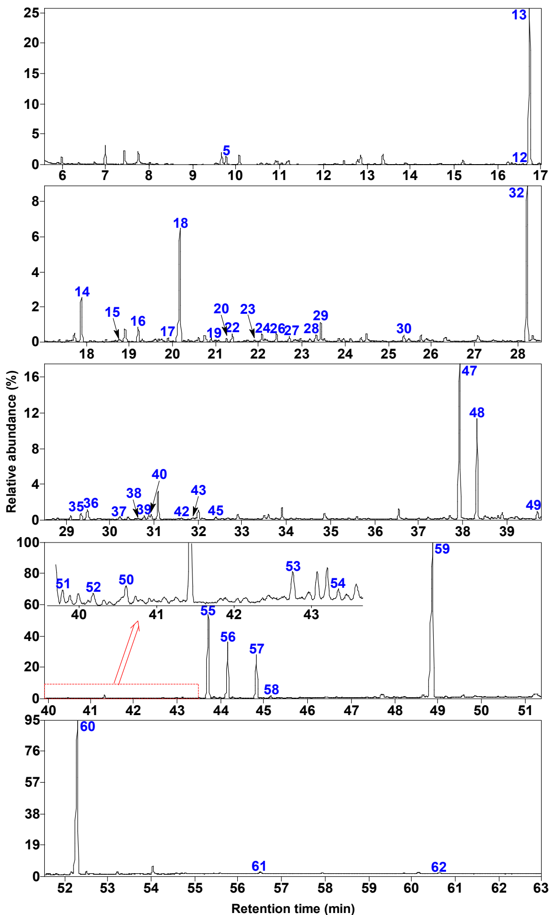
Fig. S1 Total ion chromatogram of MEIEP from RICO of ZSBC by analysis with GC/MS.
