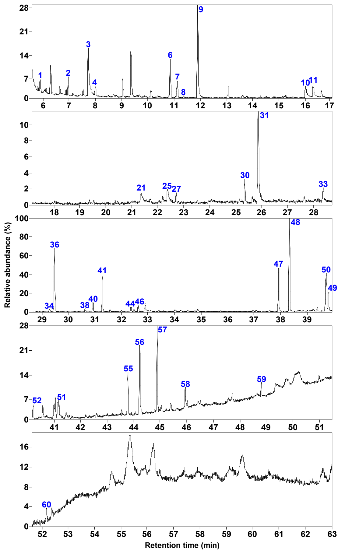
Fig. S2 Total ion chromatogram of MEEP from RICO of ZSBC by analysis with GC/MS.
