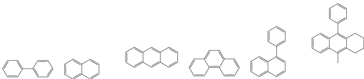
Fig. S6 Possible aromatic rings in the heavier arenepolycarboxylic acids.
