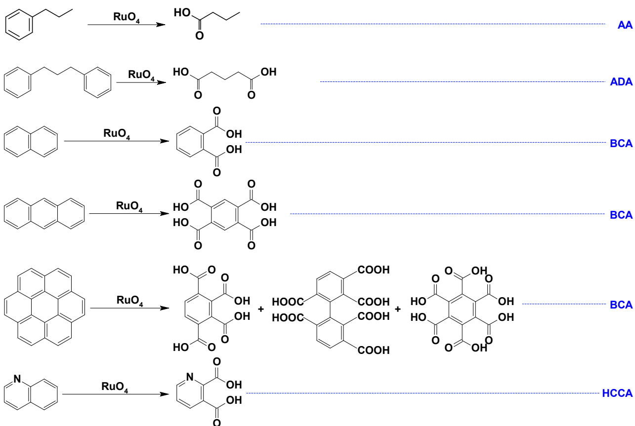
Fig. S3 Some typical reactions of RICO producing different types of oxidation products
