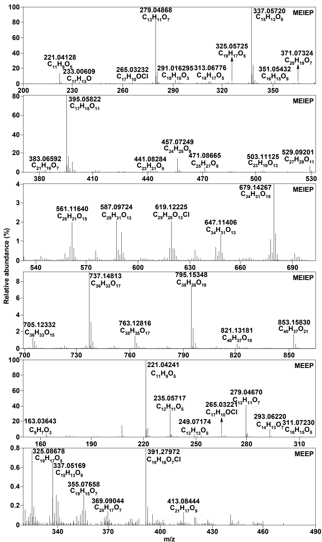
Fig. S5 Mass spectra of MEIEP and MEEP from RICO of ZSBC by analysis with ASAP/TOF-MS.
