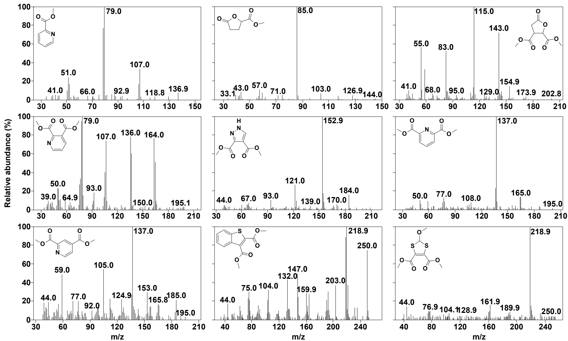
Fig. S4 Mass spectra of HCCAs from RICO of ZSBC by analysis with GC/MS.
