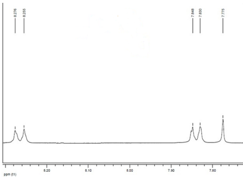
Fig.4 ^1\text{H} NMR (500MHz, \text{CDCl}_3 ) of 1-(4- nitrobenzyl)-1H-1, 2, 3-triazole (Table 2, Entry 2)
