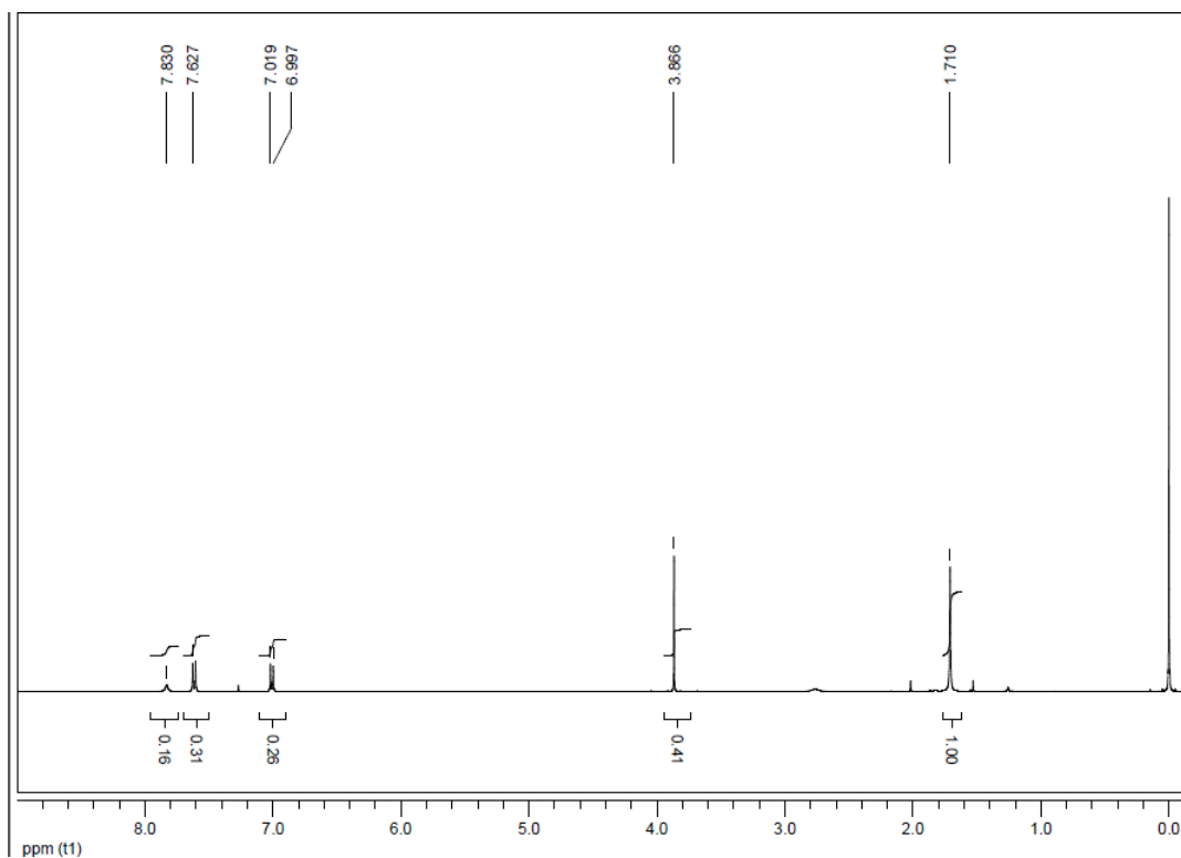
Fig.11 ^1\text{H} NMR (500MHz, \text{CDCl}_3 ) of 2-(1-(4-Methoxyphenyl)-1H-1, 2, 3-triazol-4-yl)propan-2-ol (Table 3, Entry 3)
