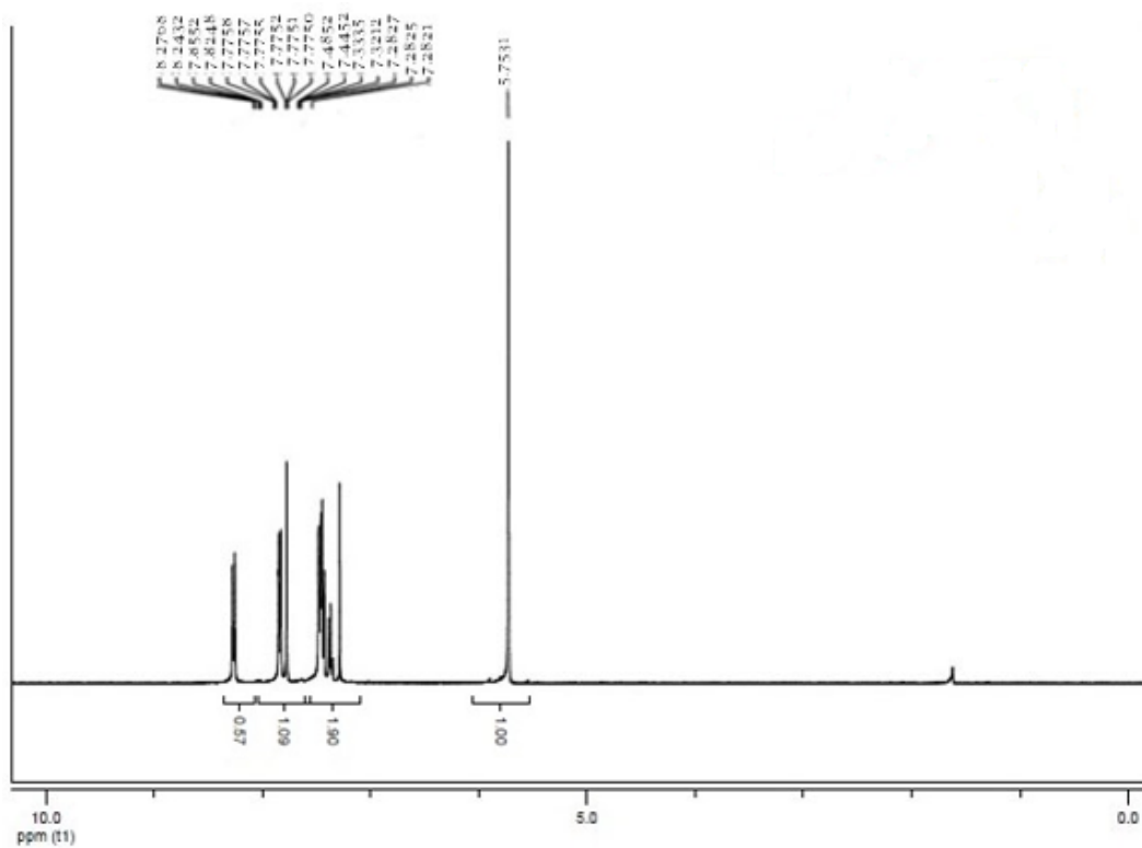
Fig.3 ^1\text{H} NMR (500MHz, \text{CDCl}_3 ) of 1-(4-nitrobenzyl)-1H-1, 2, 3-triazole (Table 2, Entry 2)
