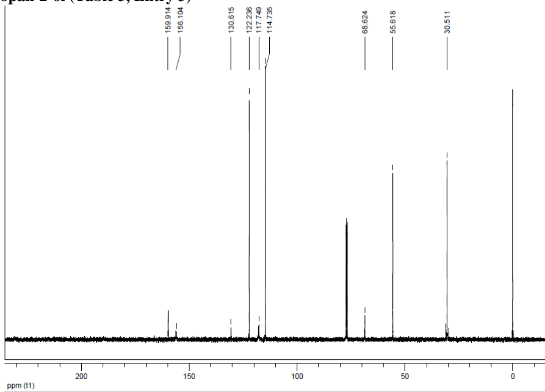
Fig.14 ^{13}\text{C} NMR (125MHz, \text{CDCl}_3 ) of 2-(1-(4-Methoxyphenyl)-1H-1, 2, 3-triazol-4-yl)propan-2-ol (Table 3, Entry 3)
