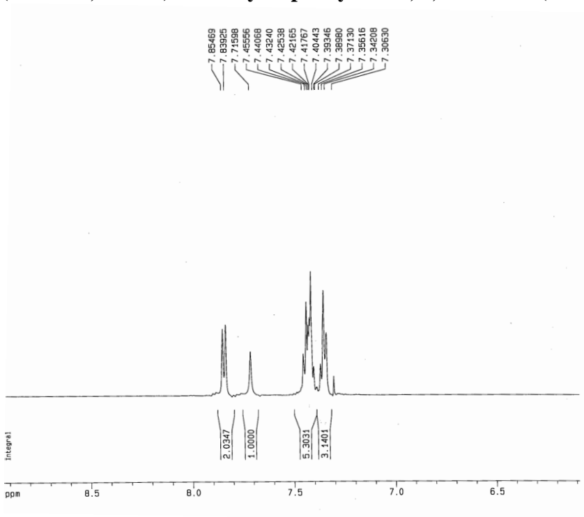
Fig.2 1 H NMR (500MHz, CDCl 3 ) of Benzyl-4-phenyl-1H-1, 2, 3-triazole (Table 2, Entry 1)
