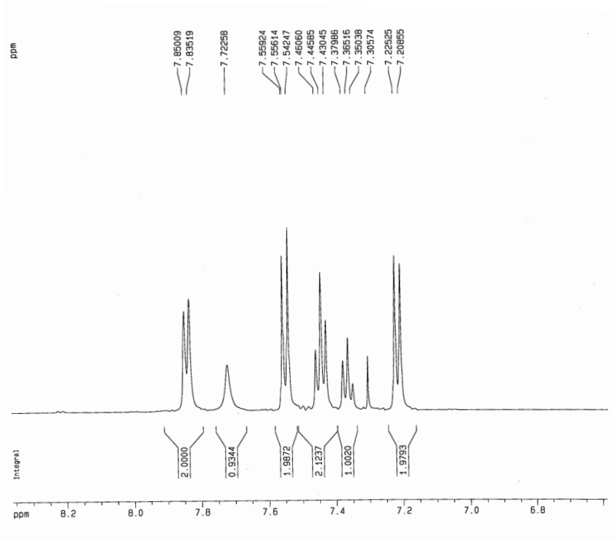
Fig.7 ^1\text{H} NMR (500MHz, \text{CDCl}_3 ) of 1-(4-bromobenzyl)-4-phenyl-1H-1, 2, 3-triazole (Table 2, Entry 6)
