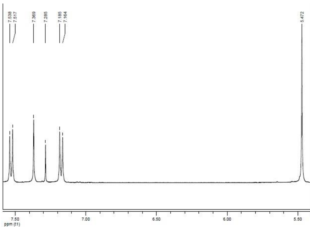
Fig.10 ^1\text{H} NMR (500MHz, \text{CDCl}_3 ) of 2-(1-(4-bromobenzyl)-1H-1,2,3-triazol-4-yl)propan-2-ol (Table 2, Entry 7)
