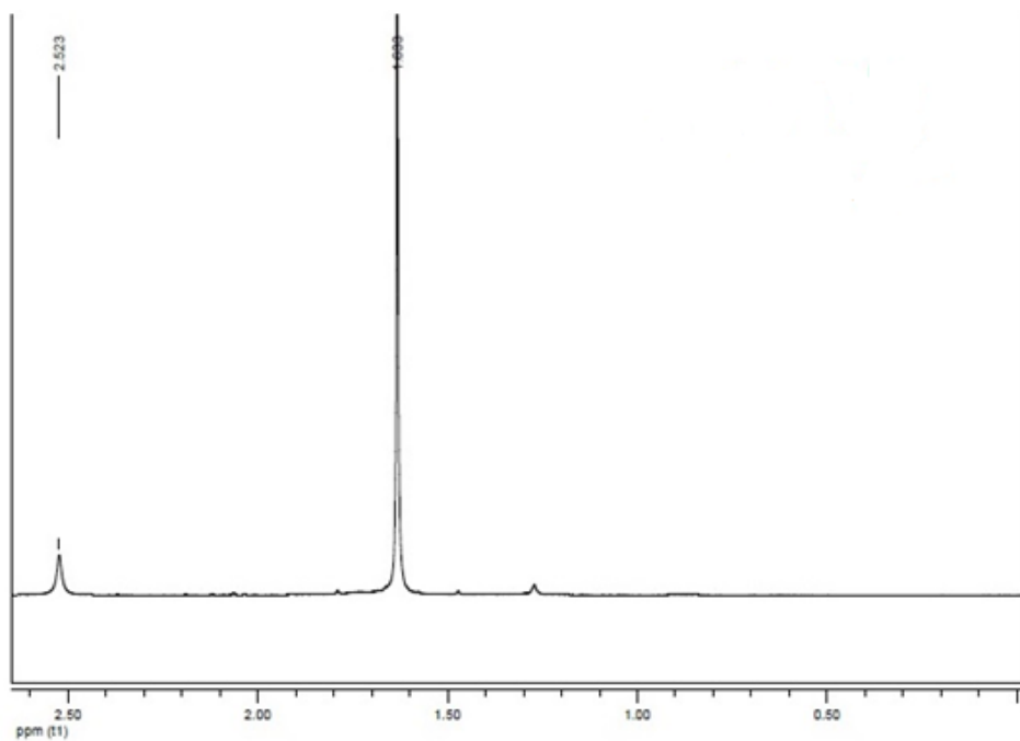
Fig.9 ^1\text{H} NMR (500MHz, \text{CDCl}_3 ) of 2-(1-(4-bromobenzyl)-1H-1,2,3-triazol-4-yl)propan-2-ol (Table 2, Entry 7)
