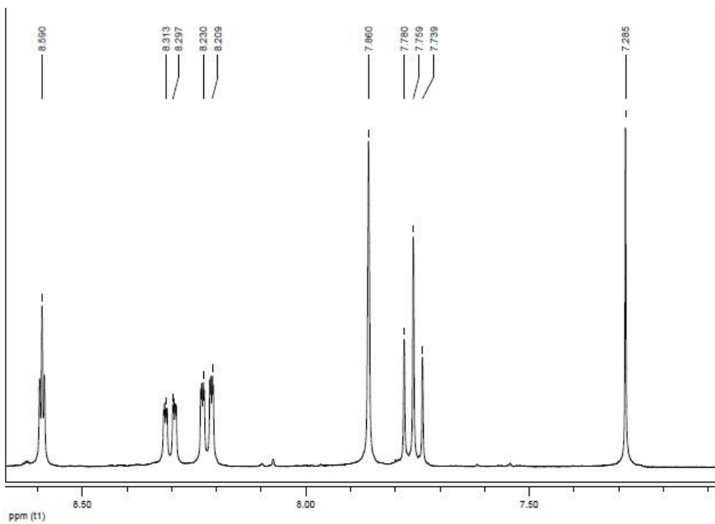
Fig.20 ^1\text{H} NMR (500MHz, \text{CDCl}_3 ) of 4-Hexyl-1-(3-nitrophenyl)-1H-1, 2, 3-triazole (Table 3, Entry 8)
