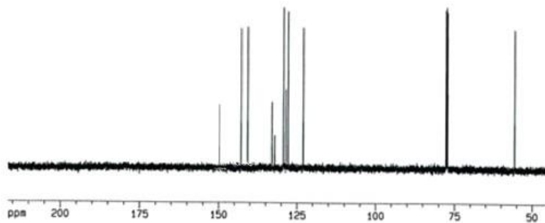
Fig.5 ^{13}\text{C} NMR (125MHz, \text{CDCl}_3 ) of 1-(4-nitrobenzyl)-1H-1,2,3-triazole (Table 2, Entry 2)
