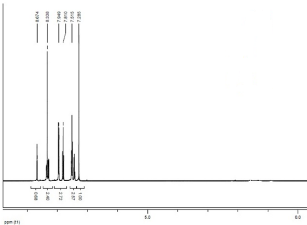
Fig.15 1 HNMR (500MHz, CDCl 3 ) of 1-(3-Nitrophenyl)-4-phenyl-1H-1, 2, 3-triazole (Table 3, Entry 7)
