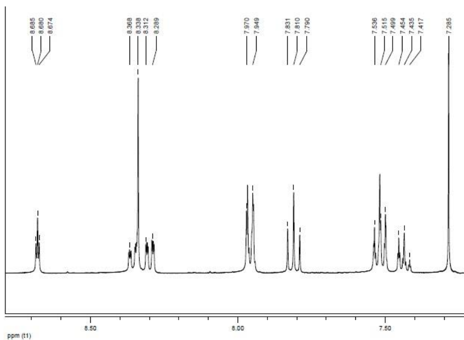
Fig.16 1 HNMR (500MHz, CDCl 3 ) of 1-(3-Nitrophenyl)-4-phenyl-1H-1, 2, 3-triazole (Table 3, Entry 7)
