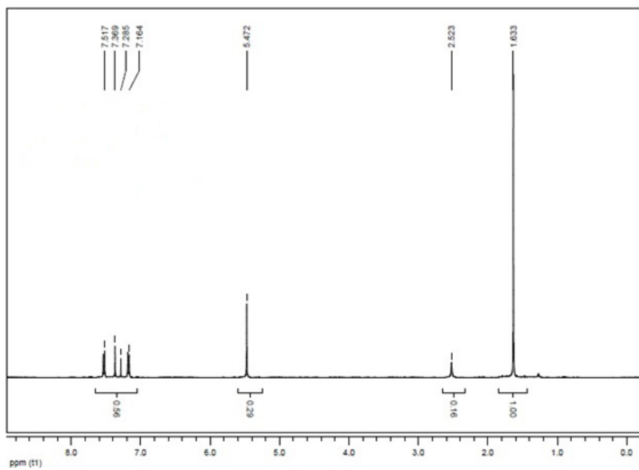
Fig.8 ^1\text{H} NMR (500MHz, \text{CDCl}_3 ) of 2-(1-(4-bromobenzyl)-1H-1, 2, 3-triazol-4-yl)propan-2-ol (Table 2, Entry 7)
