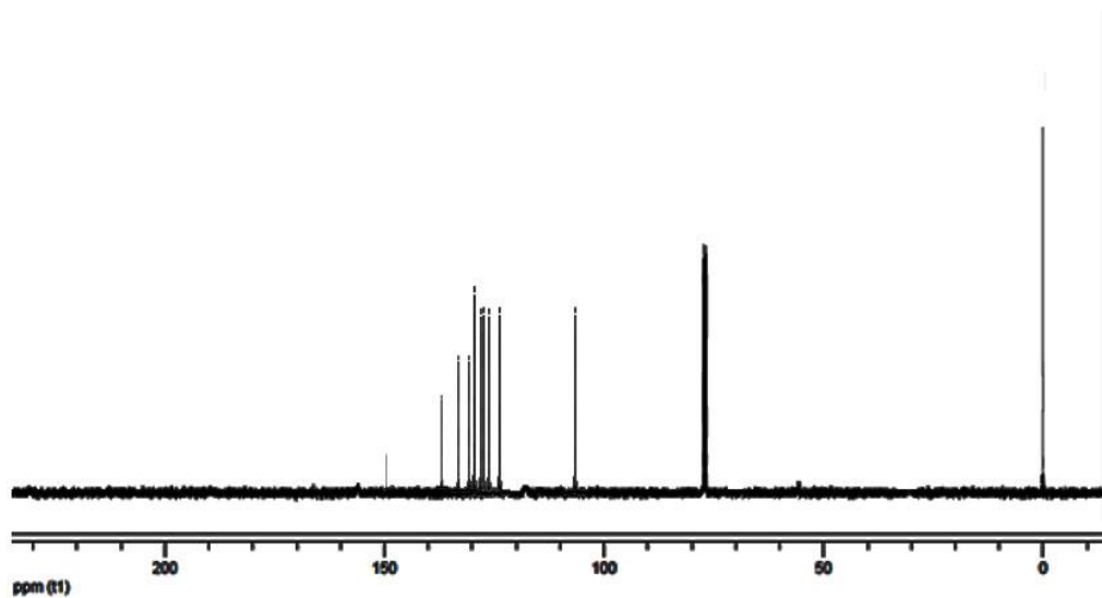
Fig.17 ^{13}\text{C} NMR (125MHz, \text{CDCl}_3 ) of 1-(3-Nitrophenyl)-4-phenyl-1H-1, 2, 3-triazole (Table 3, Entry 7)
