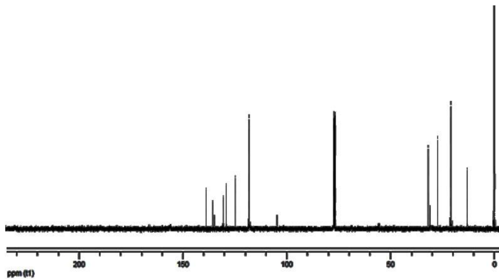
Fig.21 ^{13}\text{C} NMR (125MHz, \text{CDCl}_3 ) of 4-Hexyl-1-(3-nitrophenyl)-1H-1, 2, 3-triazole (Table 3, Entry 8)
