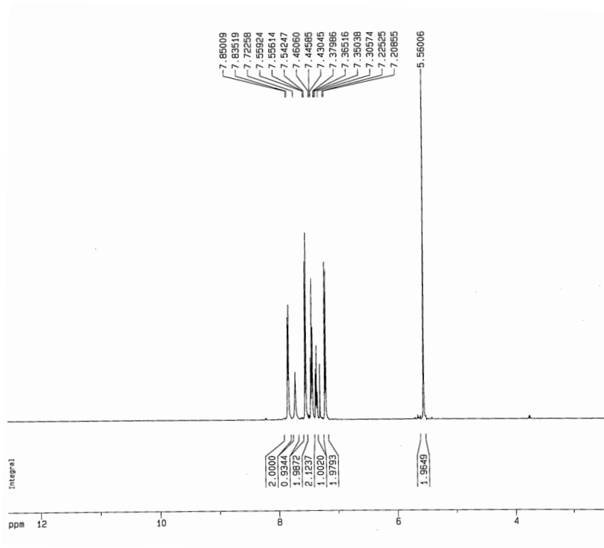
Fig.6 ^1\text{H} NMR (500MHz, \text{CDCl}_3 ) of 1-(4-bromobenzyl)-4-phenyl-1H-1,2,3-triazole (Table 2, Entry 6)
