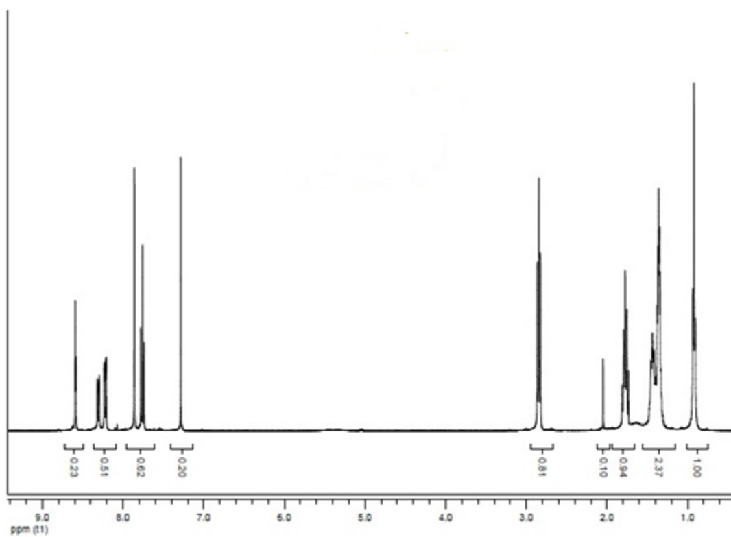
Fig.18 ^1\text{H} NMR (500MHz, \text{CDCl}_3 ) of 4-Hexyl-1-(3-nitrophenyl)-1H-1, 2, 3-triazole (Table 3, Entry 8)
