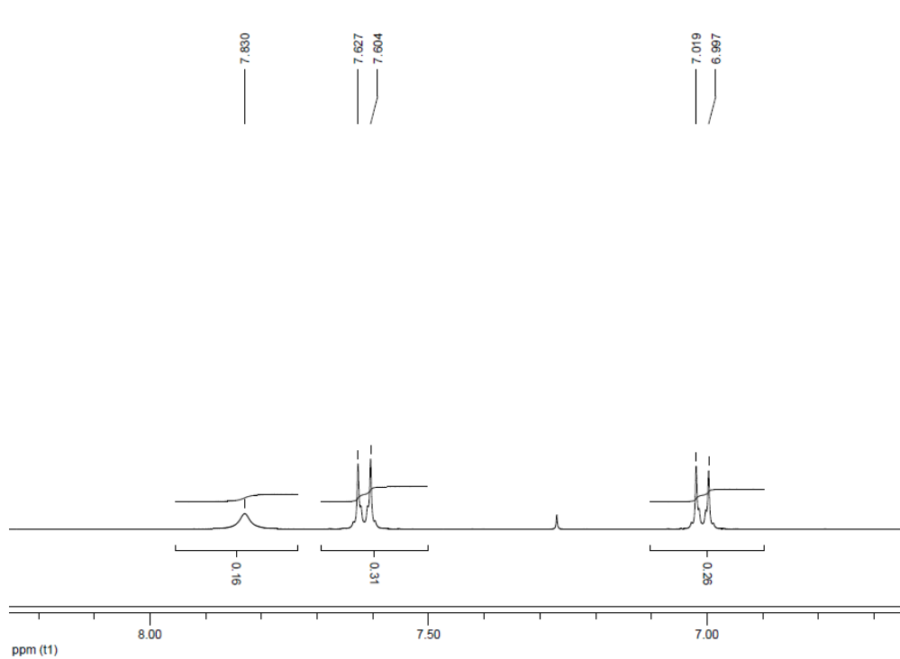
Fig.13 ^1\text{H} NMR (500MHz, \text{CDCl}_3 ) of 2-(1-(4-Methoxyphenyl)-1H-1, 2, 3-triazol-4-yl)propan-2-ol (Table 3, Entry 3)
