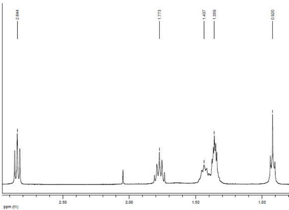
Fig.19 ^1\text{H} NMR (500MHz, \text{CDCl}_3 ) of 4-Hexyl-1-(3-nitrophenyl)-1H-1, 2, 3-triazole (Table 3, Entry 8)
