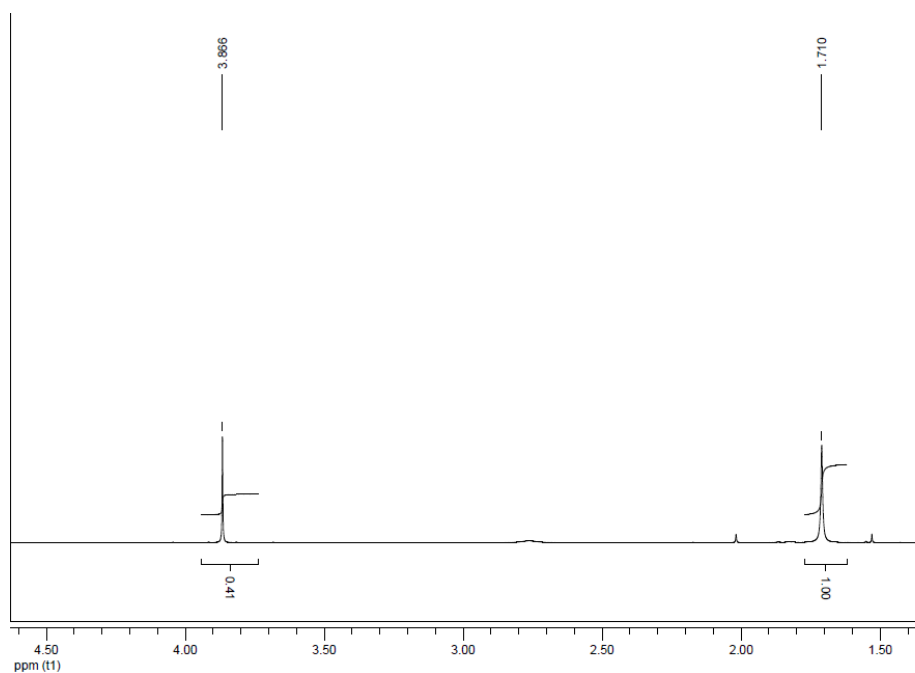
Fig.12 ^1\text{H} NMR (500MHz, \text{CDCl}_3 ) of 2-(1-(4-Methoxyphenyl)-1H-1, 2, 3-triazol-4-yl)propan-2-ol (Table 3, Entry 3)
