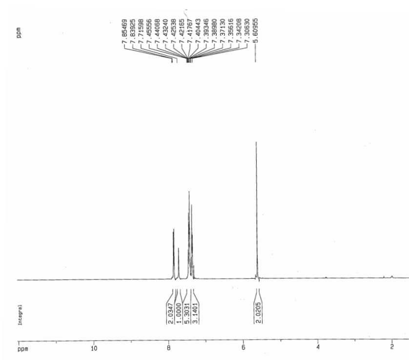
Fig.1 1 H NMR (500MHz, CDCl 3 ) of Benzyl-4-phenyl-1H-1, 2, 3-triazole (Table 2, Entry 1)
