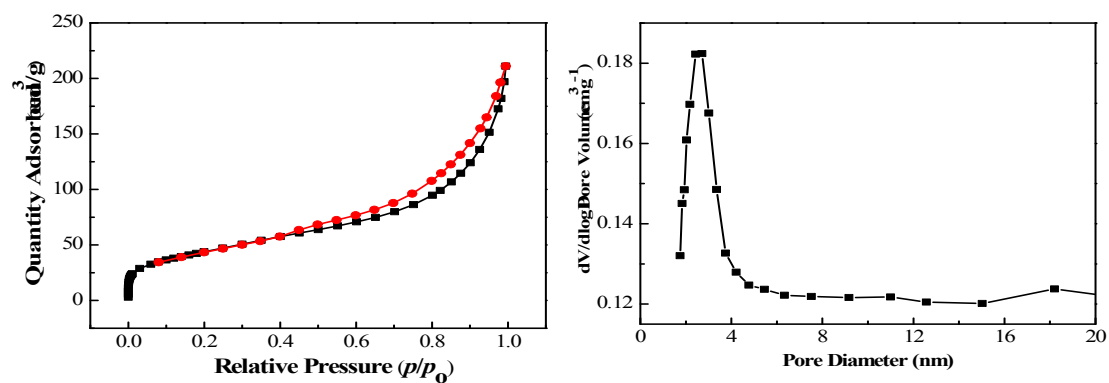
Fig.6. The BET of \text{SO}_4^{2-}/\text{WO}_x\text{-ZrO}_2
