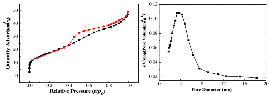
Fig.5. The BET of \text{MoO}_x\text{-ZrO}_2
