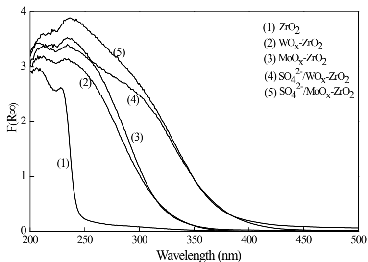
Fig. 1. UV-vis DRS of different catalysts
