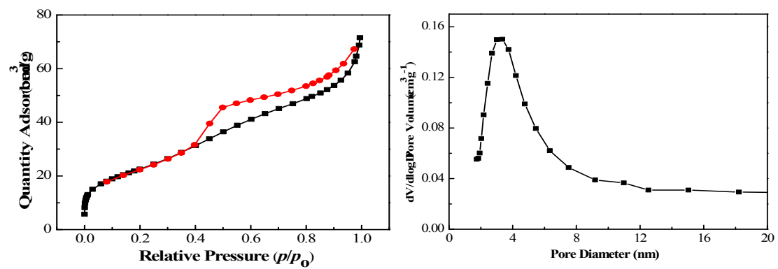
Fig.7. The BET of \text{SO}_4^{2-}/\text{MoO}_x\text{-ZrO}_2
