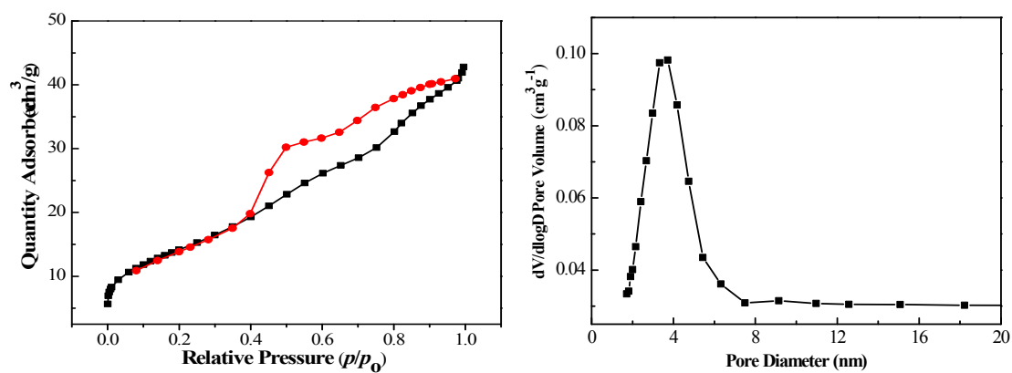
Fig.3. The BET of \text{ZrO}_2
