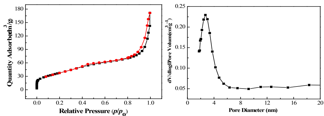
Fig.4. The BET of \text{WO}_x\text{-ZrO}_2
