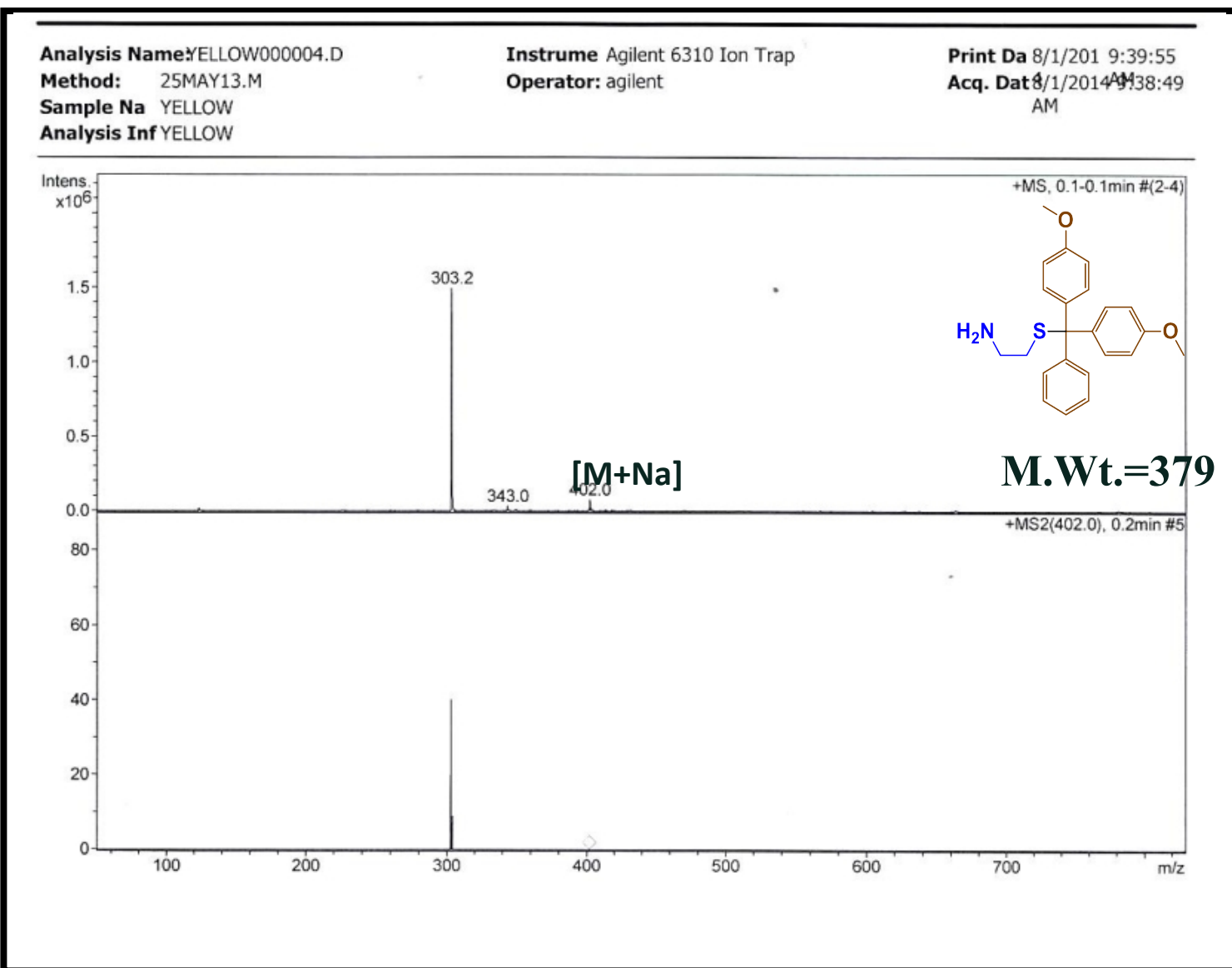
Mass spectrum of Cysteamine-DMT
