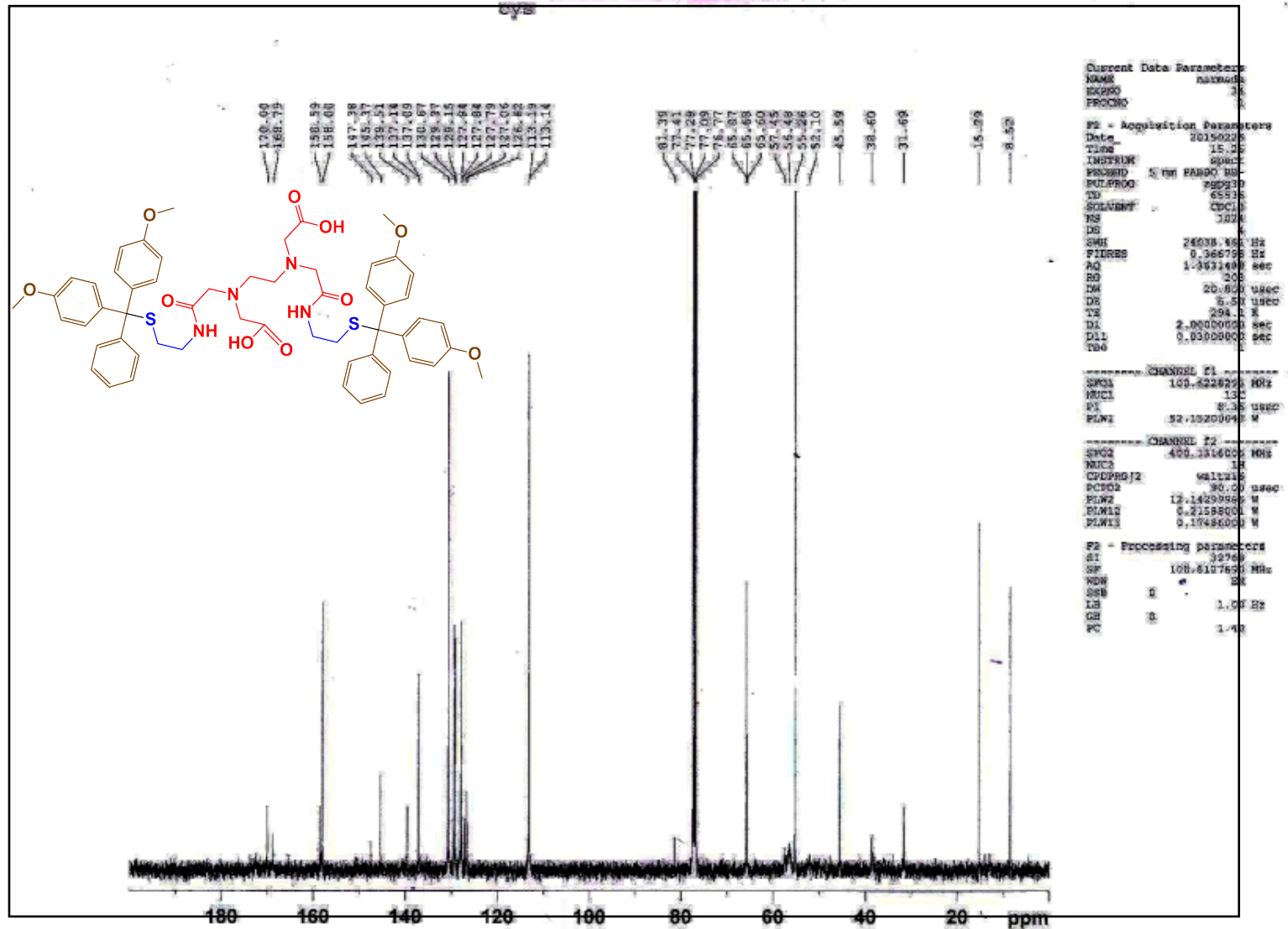
^{13}\text{C} NMR of EDTA-Bis-Cysteamine-DMT
