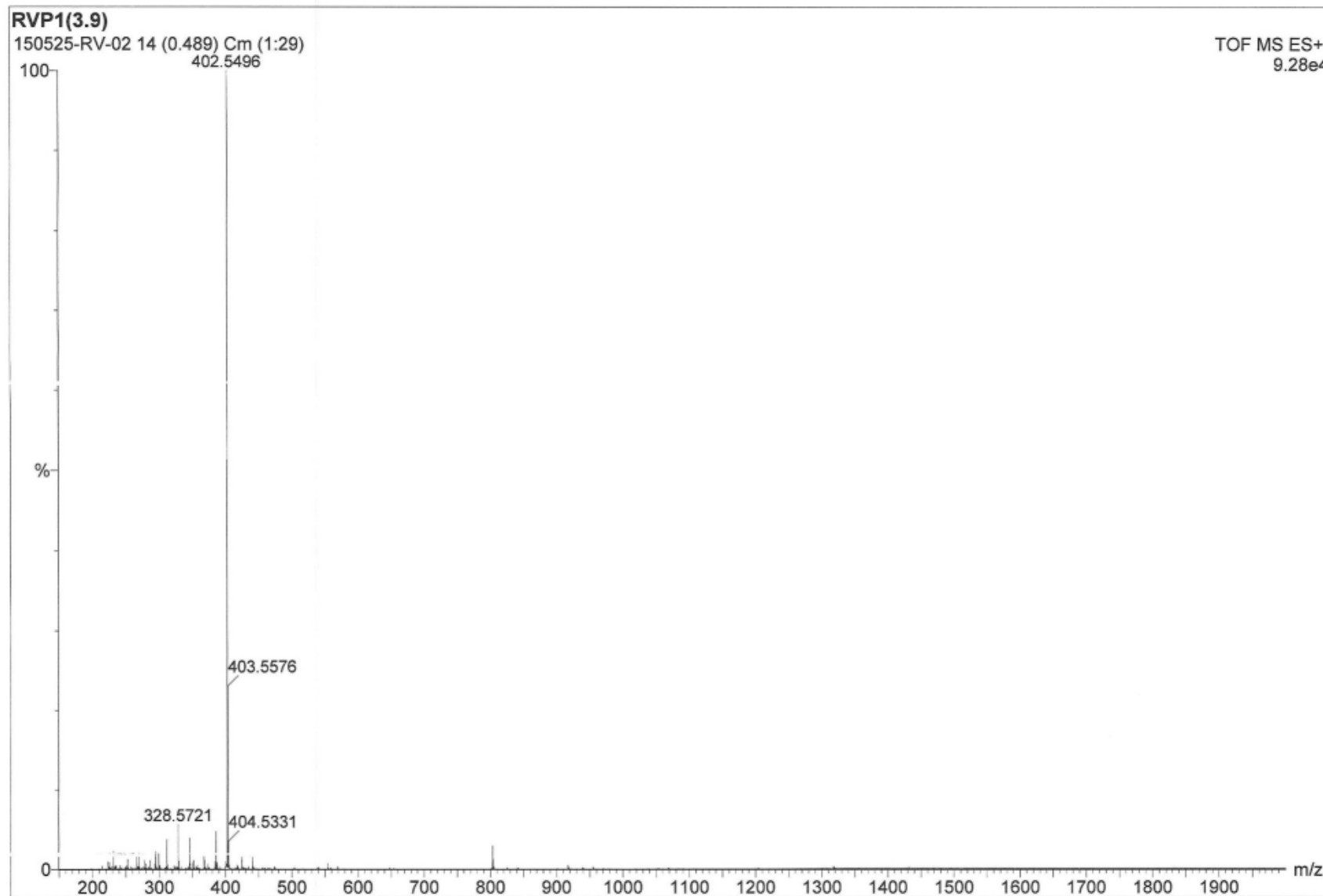
HRMS of GNDR peptide
