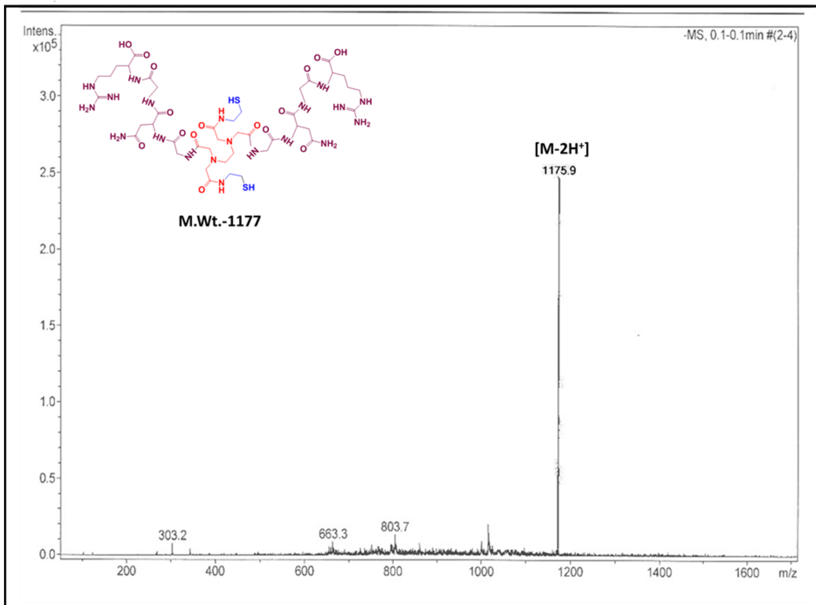
Mass Spectrum of EDTA-Bis-GNGR ligand
