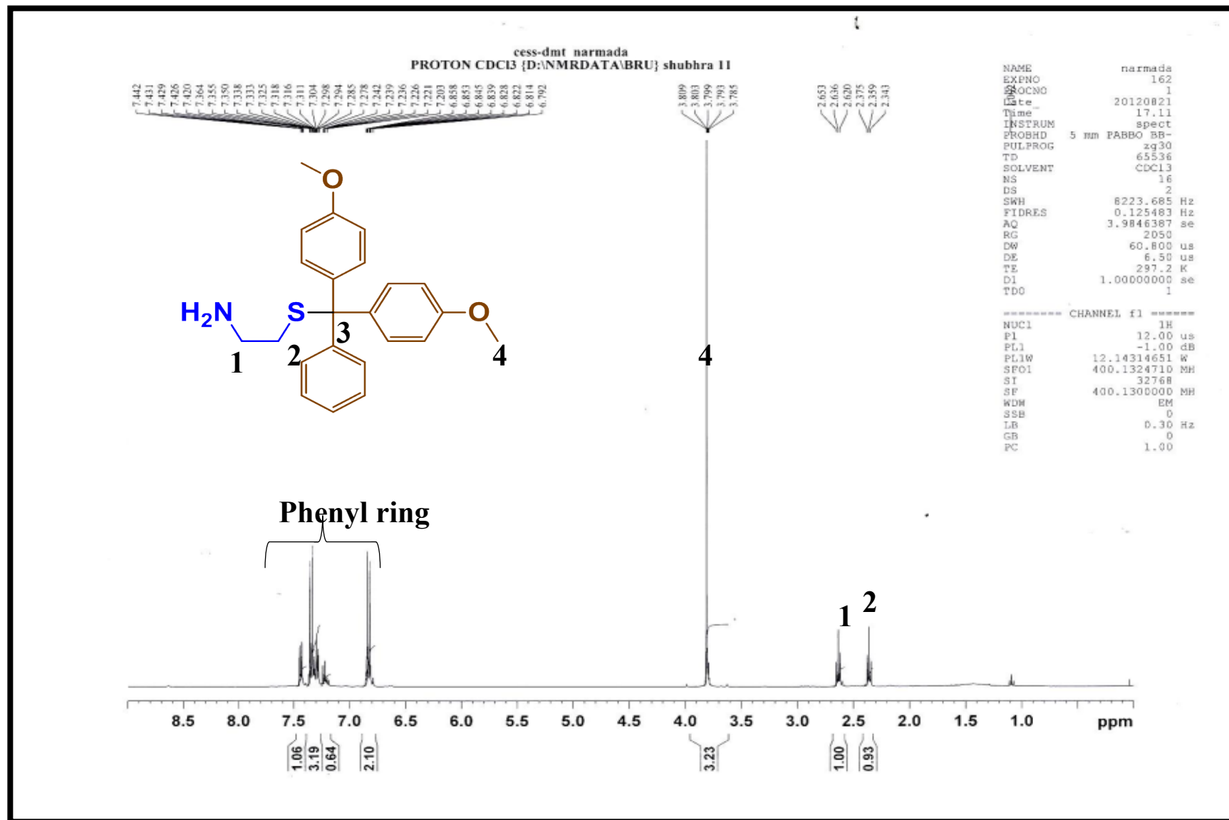
1 H-NMR spectrum of Cysteamine-DMT
