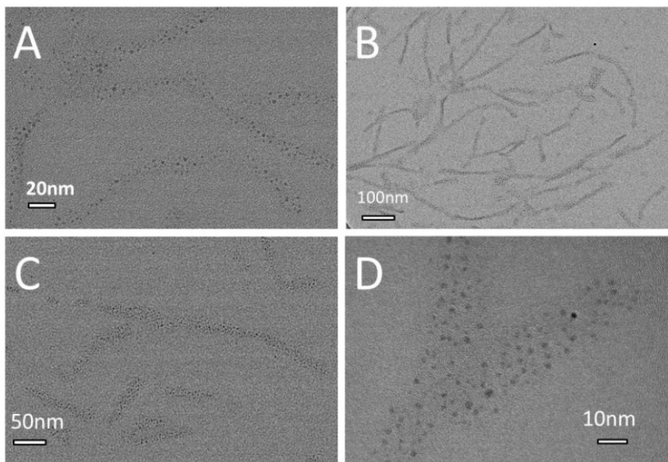
Fig. S3. TEM images of Ag NCs-a3 (A, B) and Ag NCs-a2 (C, D).
