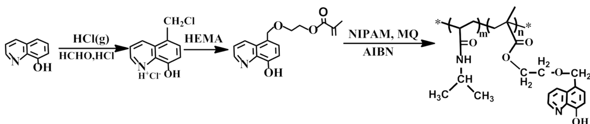
Fig.S1. Synthetic route of CPL.
