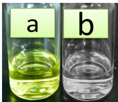
Fig. S4. Digital images of 4-nitrophenol before (a) and after (b) reduction.
