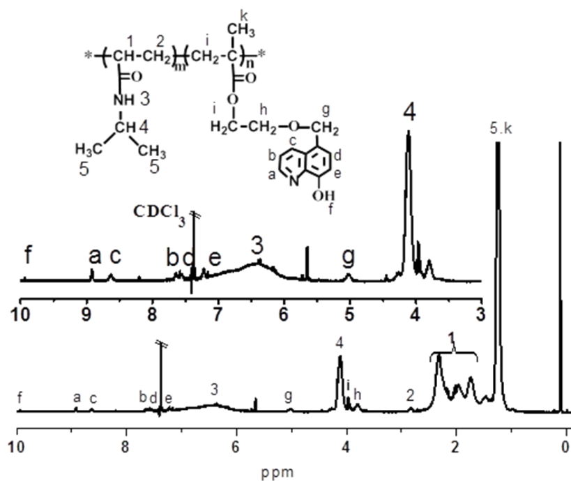
Fig. S2. 1 H-NMR spectra of CPL in CDCl 3 .
