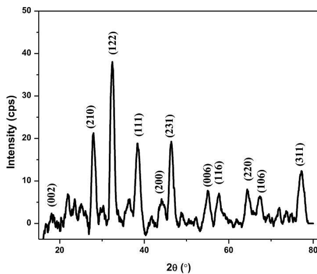
Fig. S1. XRD pattern of PLGA/Ag NC. The pattern of PLGA/Ag NC matches the face centered cubic (FCC) structure of bulk silver.
